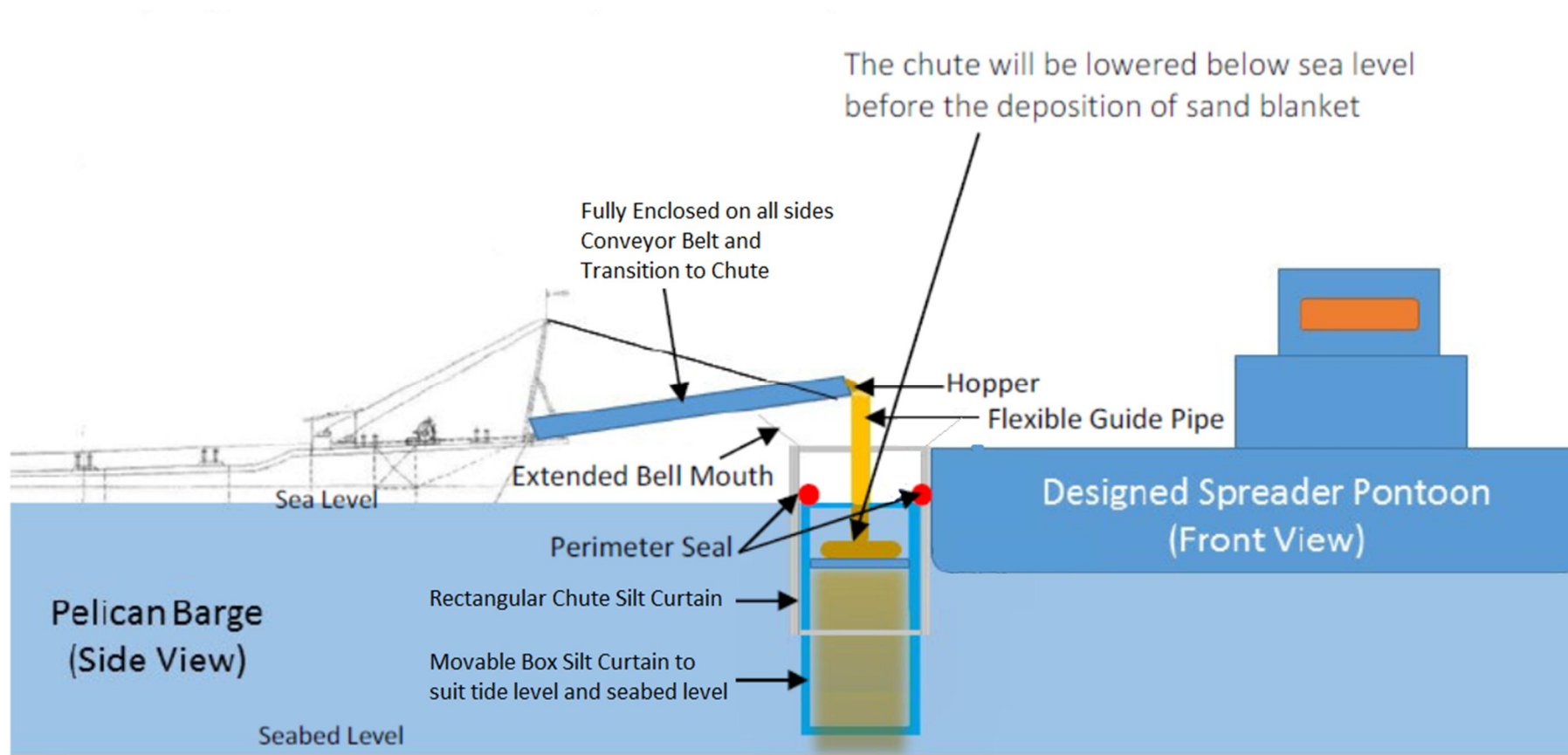
Figure B.5: Illustration of Cage-Type Silt Curtain comprising Rectangular Chute and Movable Box
