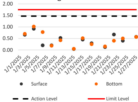
Turbidity (Depth-Averaged) during Mid-Ebb
