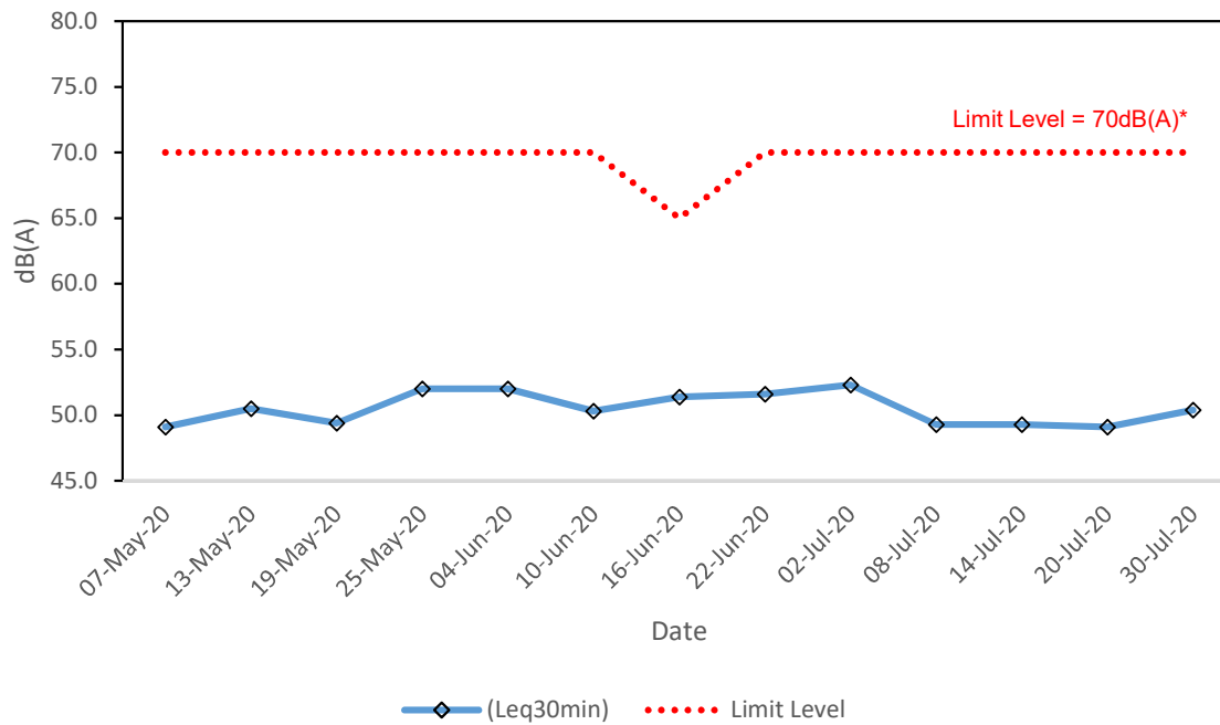
Noise Level for 30 min, dB(A), at NM2
