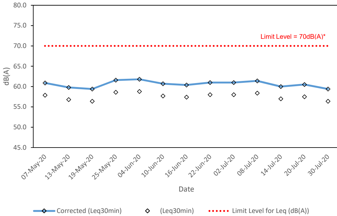
Noise Level for 30 min, dB(A), at NM1A
