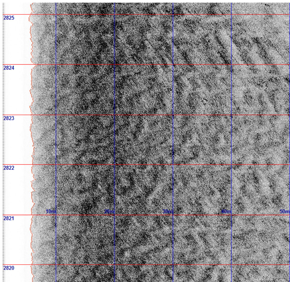
(a) Seabed sand ripples in Segment A
