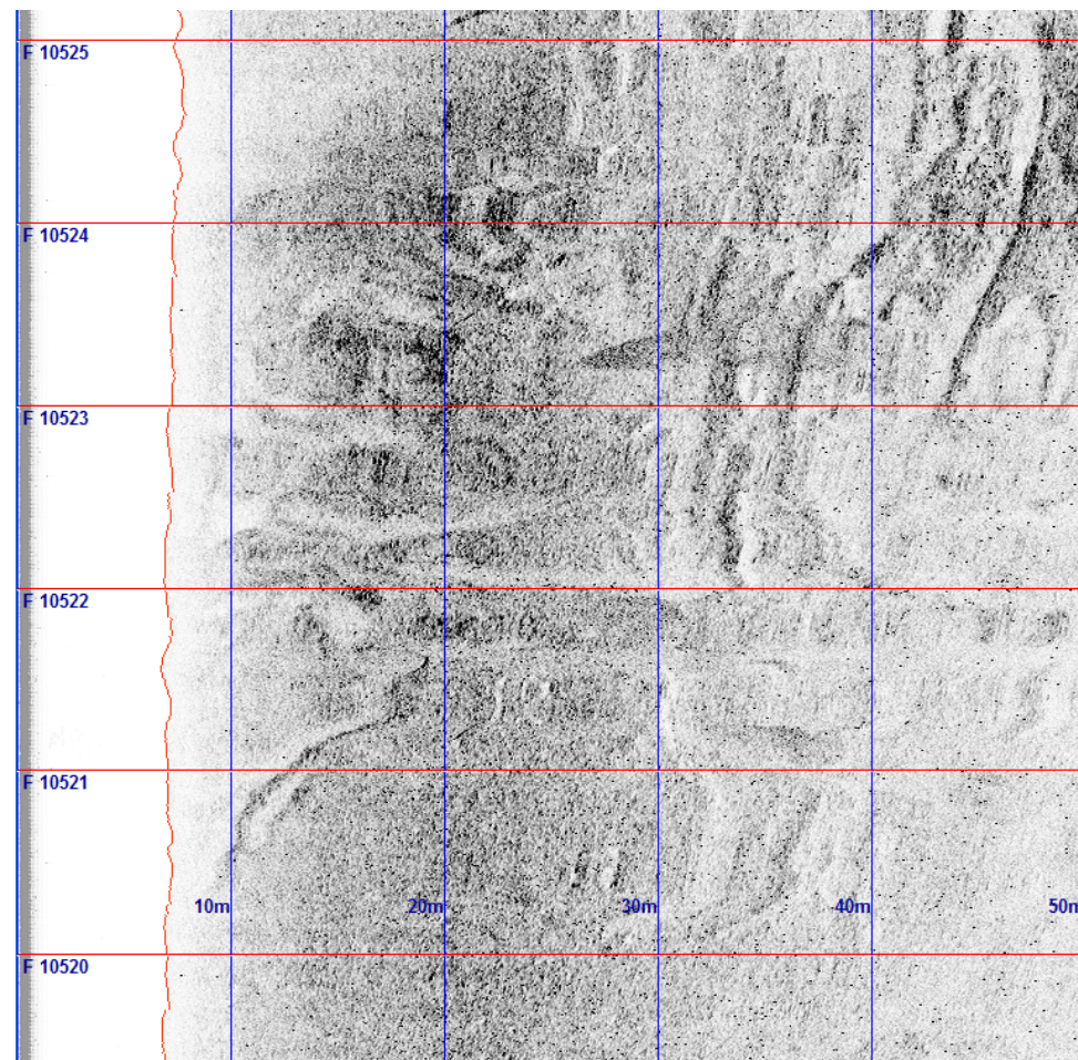
(b) Seabed impacted by trawling in Segment F
