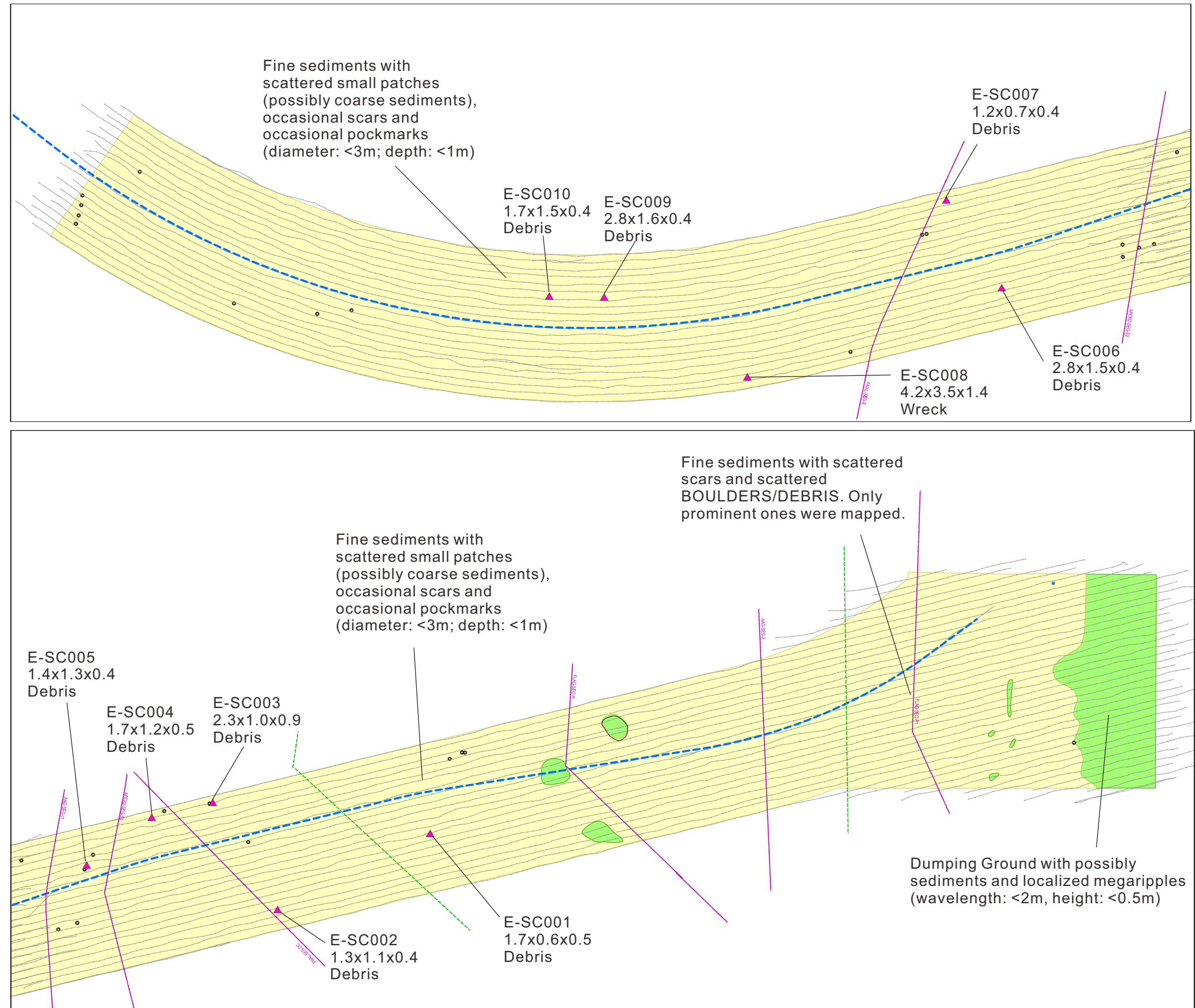
Survey Track Plots, Seabed Features and Sonar Contacts Locations in Segment E
