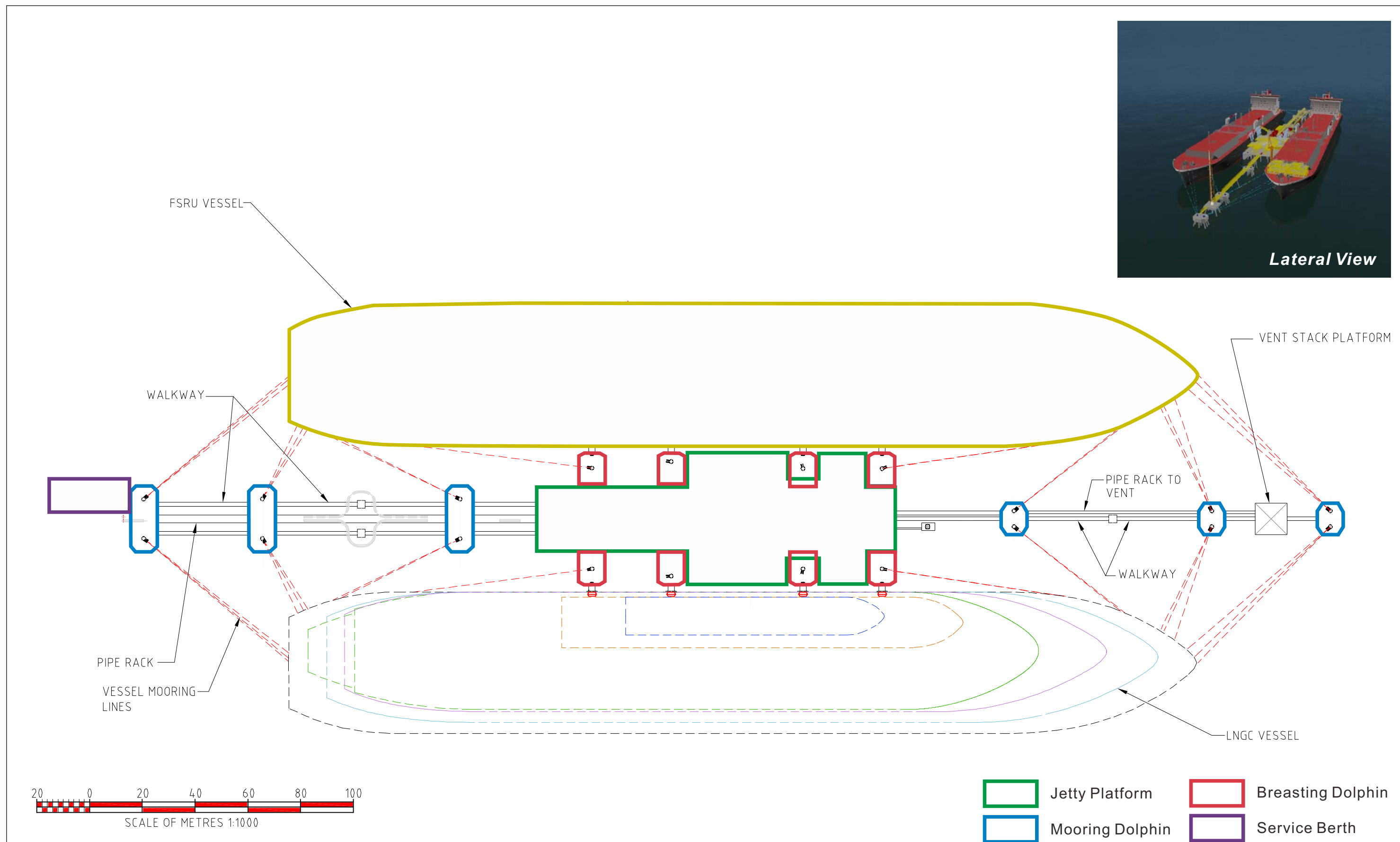
Figure 3.5 Conceptual Layout of the LNG Terminal Environmental Resources Management ERM FILE: 0359722o2.cdr DATE: 12/03/2018
