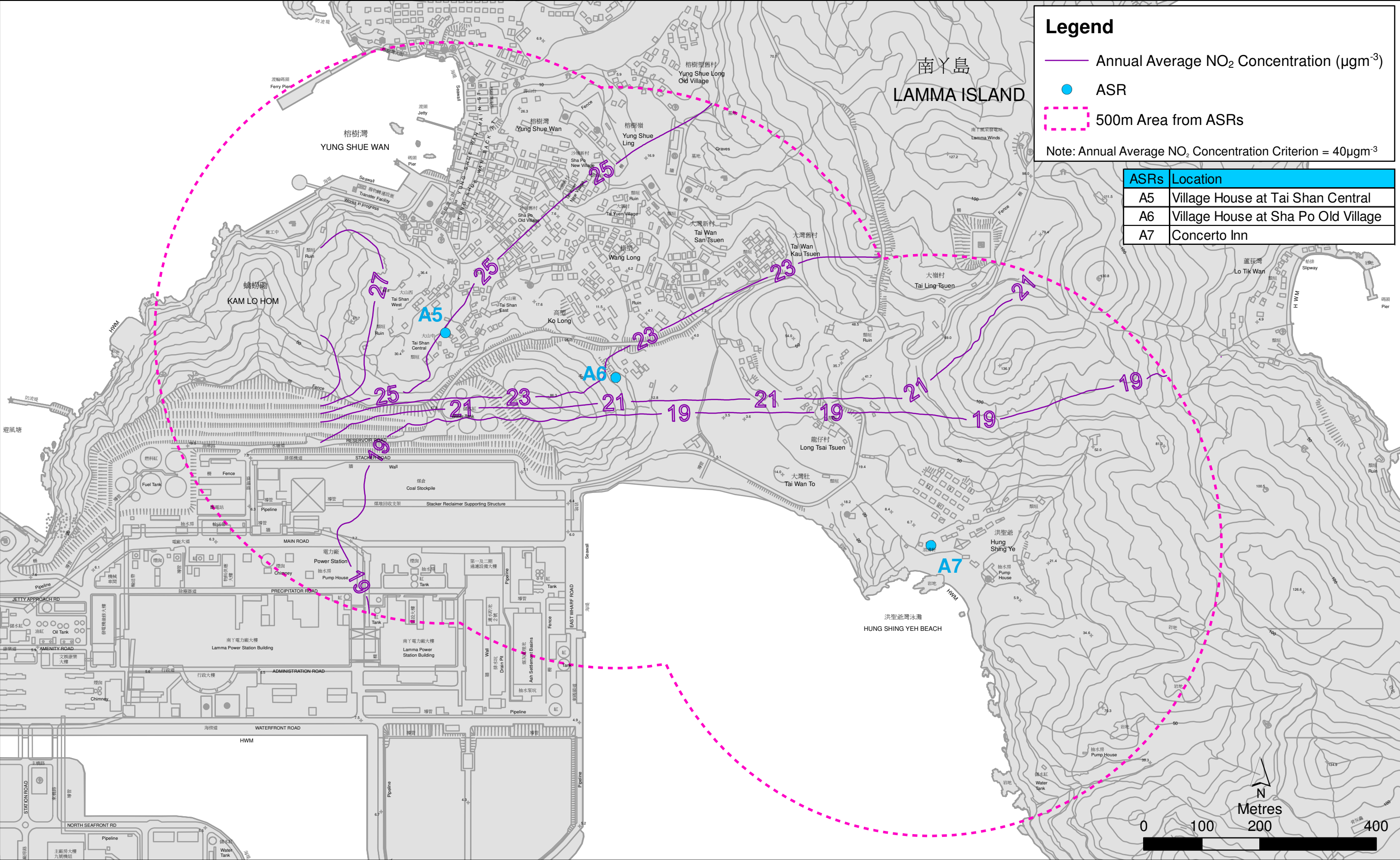
Figure 4.15 Contour of Cumulative Annual Average NO 2 Concentration at 10m above ground in the LPS area
