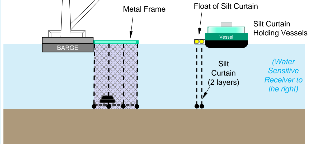
(b) Cross-Section of Silt Curtain Arrangement
