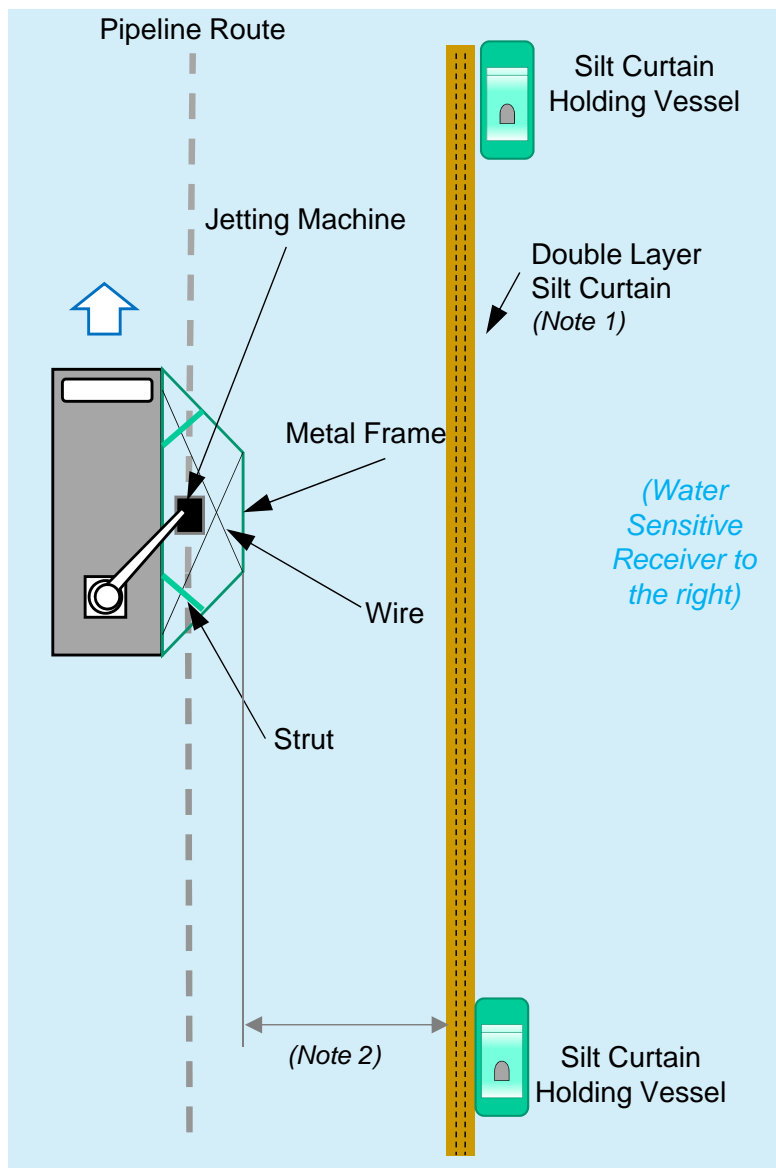
Not to Scale (a) Plan of Silt Curtain Arrangement
