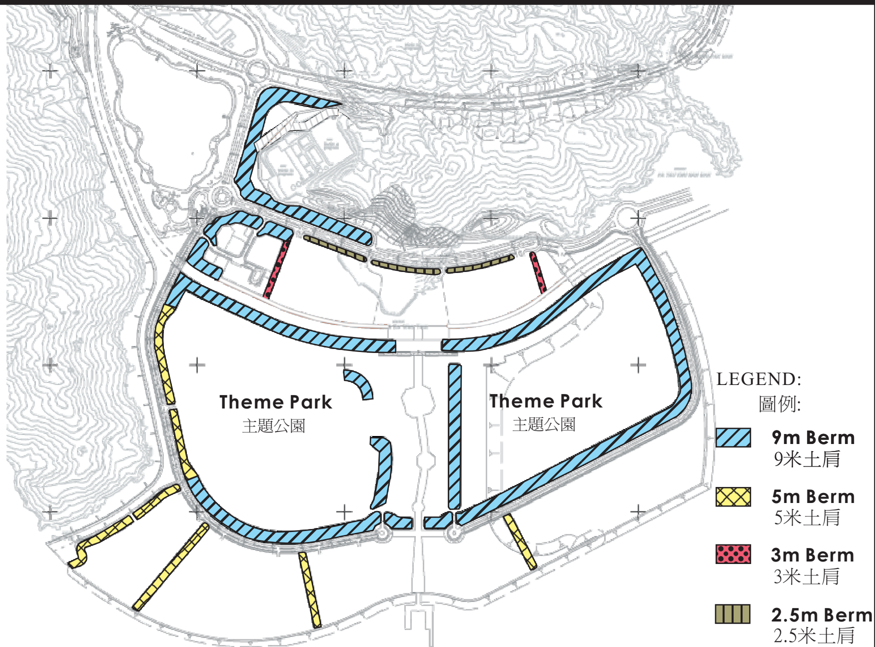
Figure 6 Location of Earth Berms in the Project
