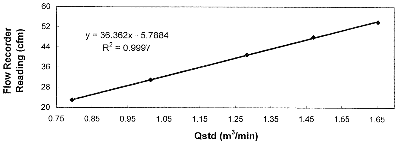
Sampler 9503 Calibration Curve Site: Tuen Mun 38 (TM-A1) Date of Calibration: 10 July 2008
