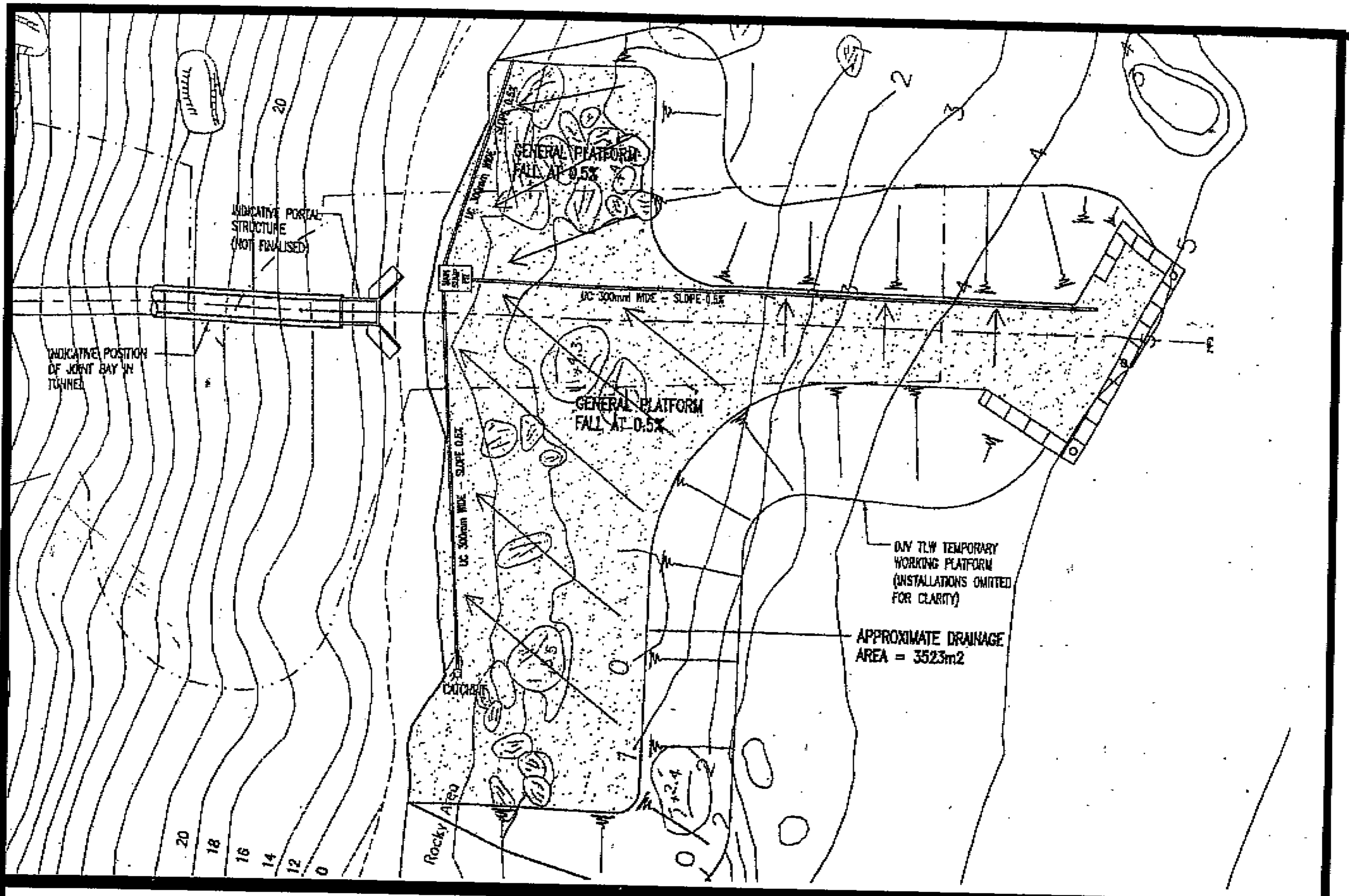
Figure 8 Schematic Layout of Construction Site Drainage System at Tai Long Wan
