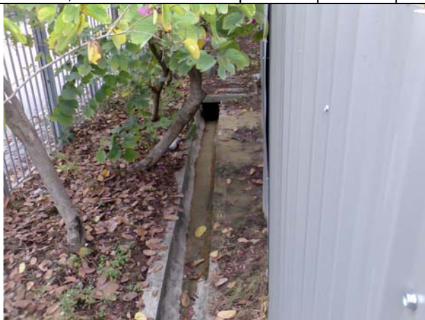
Photo 3: Turbidity water discharged to the u-channel was observed at Ha Tsuen PS, the contractor was reminded to provide sand bags to divert the surface runoff to de-silting facility.
