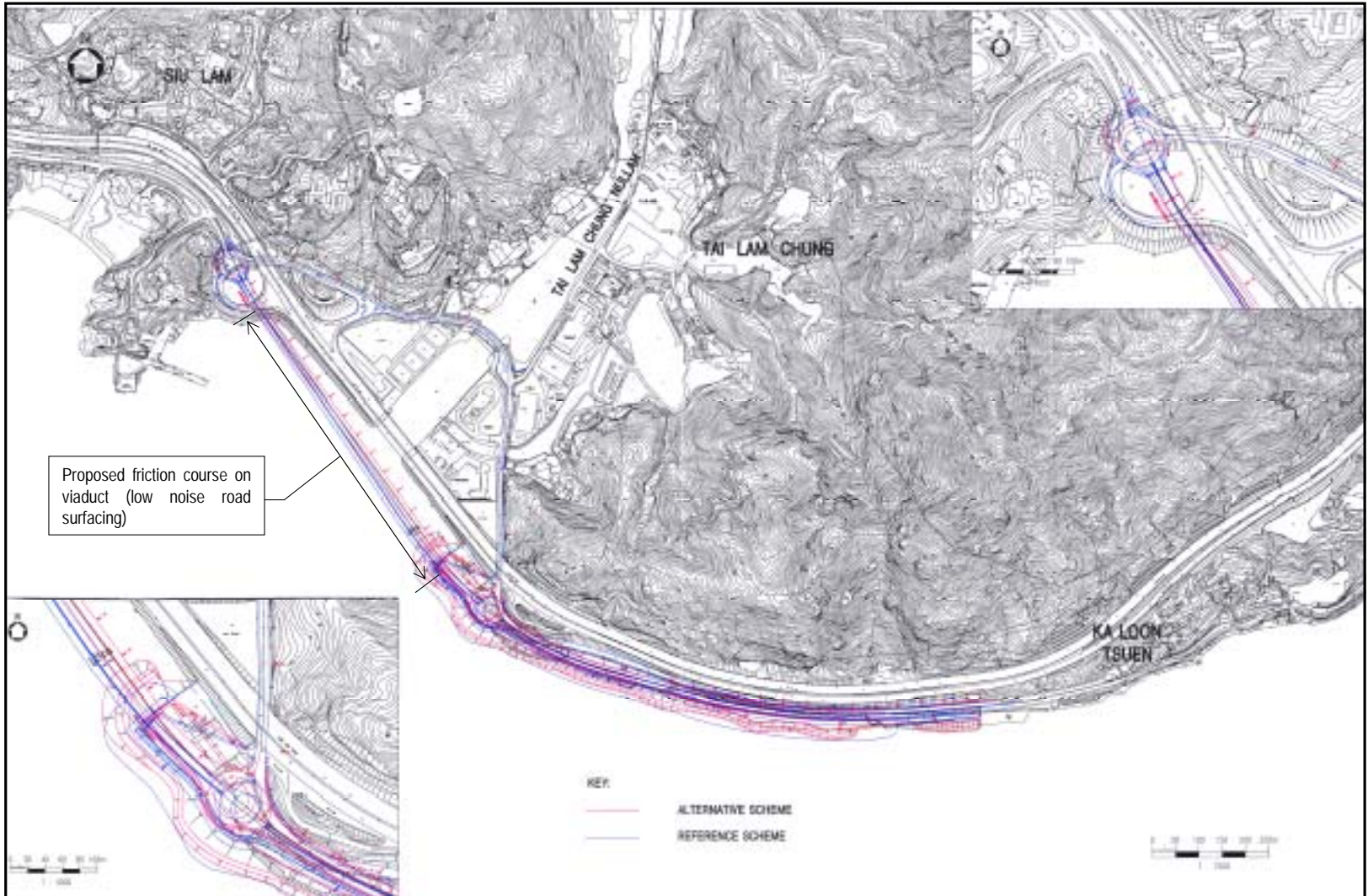
Improvement to Castle Peak Road Between Ka Loon Tsuen and Siu Lam – Proposed Alternative Scheme
