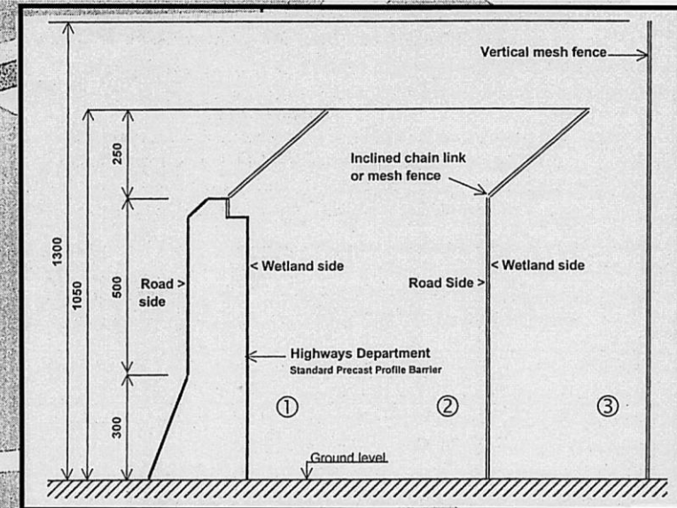
Options for proposed mammal barrier
