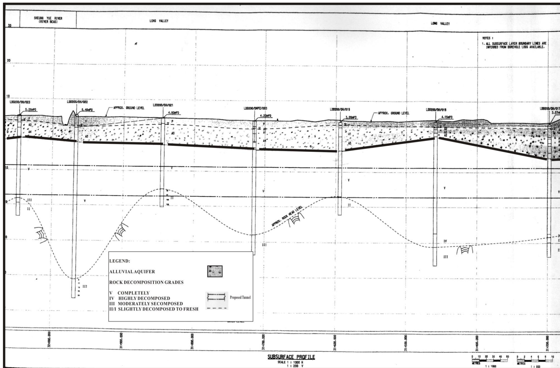
Figure 3 - Sheung Shui to Lok Ma Chau Spur Line (上水至落馬洲支線) 圖三 - 條例3.12所指貫穿塱原之隧道垂直側面圖 (Reproduced from Figure 1 of Appendix A3.1 (Volume 3 of 5) of the EIA Report (Register No.: AEIAR-052/2002) 摘自環評報告第三冊附件A3.1圖一 (登記冊編號: AEIAR-052/2002)
