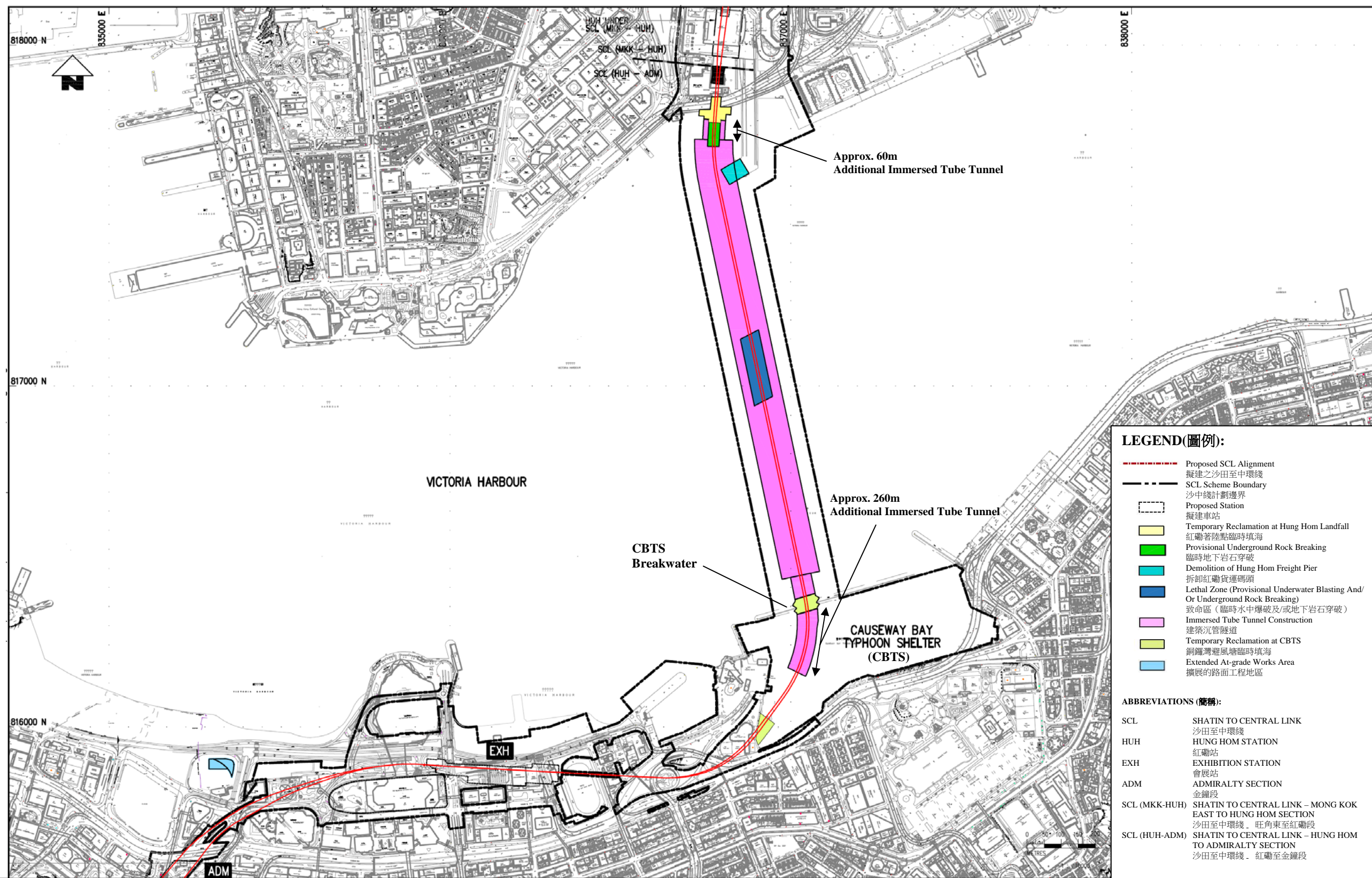
Figure 2: Marine Works for Shatin to Central Link – Hung Hom to Admiralty Section within Victoria Harbour 圖 沙田至中環綫 - 紅磡至金鐘段在維多利亞港內之海上工程
