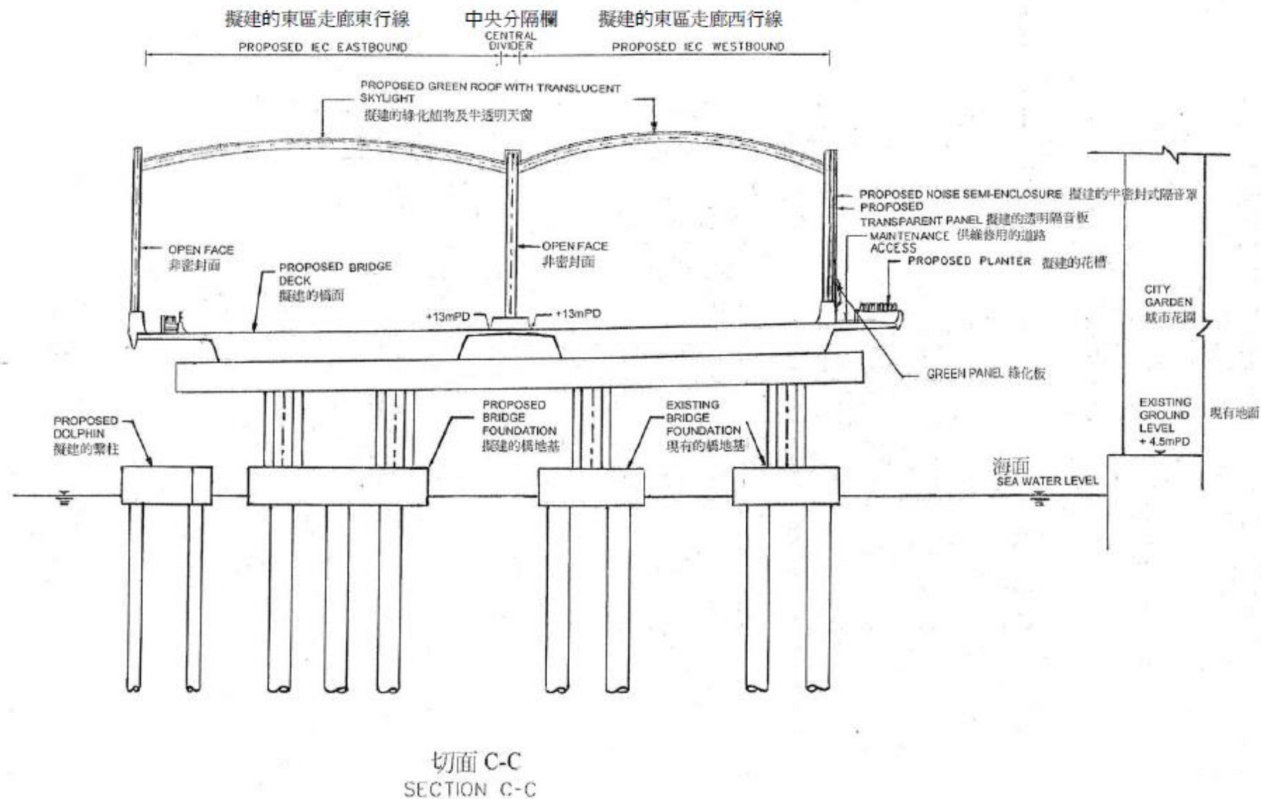
Figure 4f: Section of Direct Noise Mitigation Measures 圖 4f: 直接噪音緩解措施切面圖
