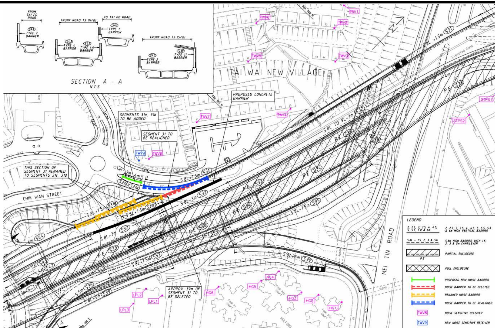
Figure 12 : Details of Noise Barriers segment nos. S31,S31a,S31b,S31c and S31d near Tai Wai New Village
