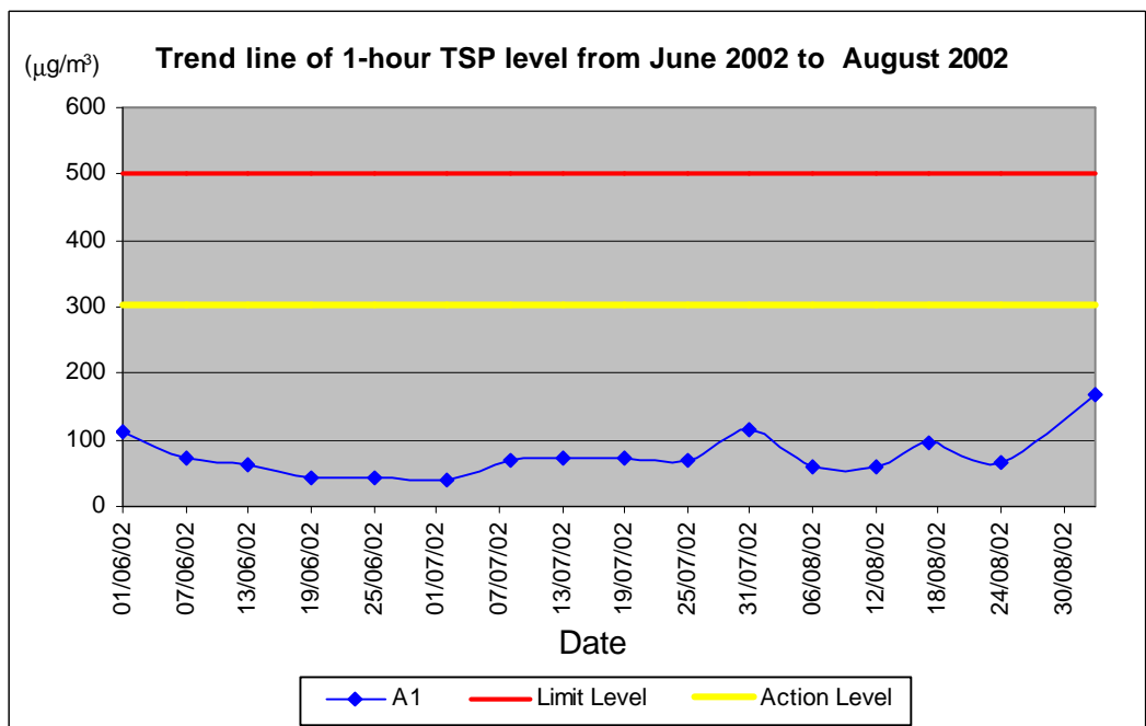
Figure 5-2 Trend of 1-hour TSP levels from June 2002 to August 2002
