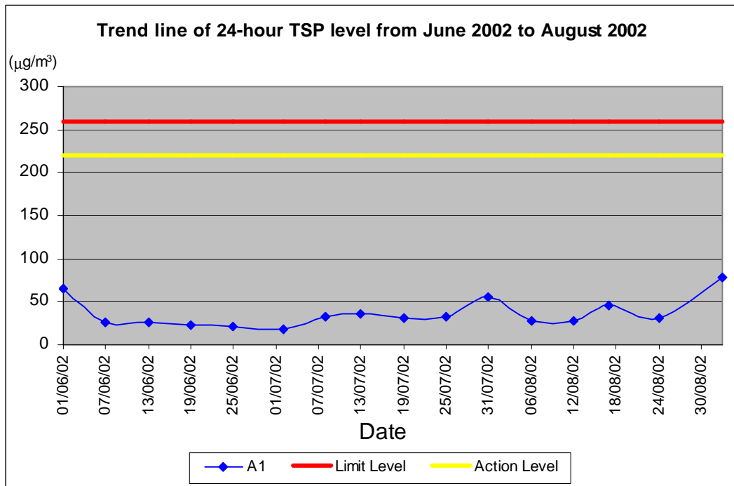
Figure 5-1 Trend of 24-hour TSP levels from June 2002 to August 2002
