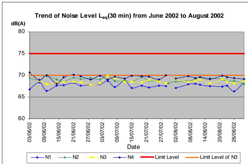
Figure 4-1 Trend of noise monitoring level from June 2002 to August 2002
