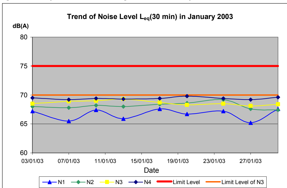
Figure 4-1 Daytime noise monitoring results for January 2003
