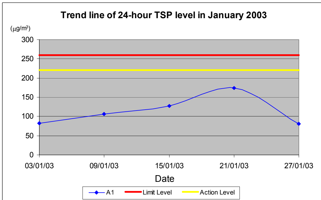
Figure 5-1 24-hour TSP monitoring results for January 2003
