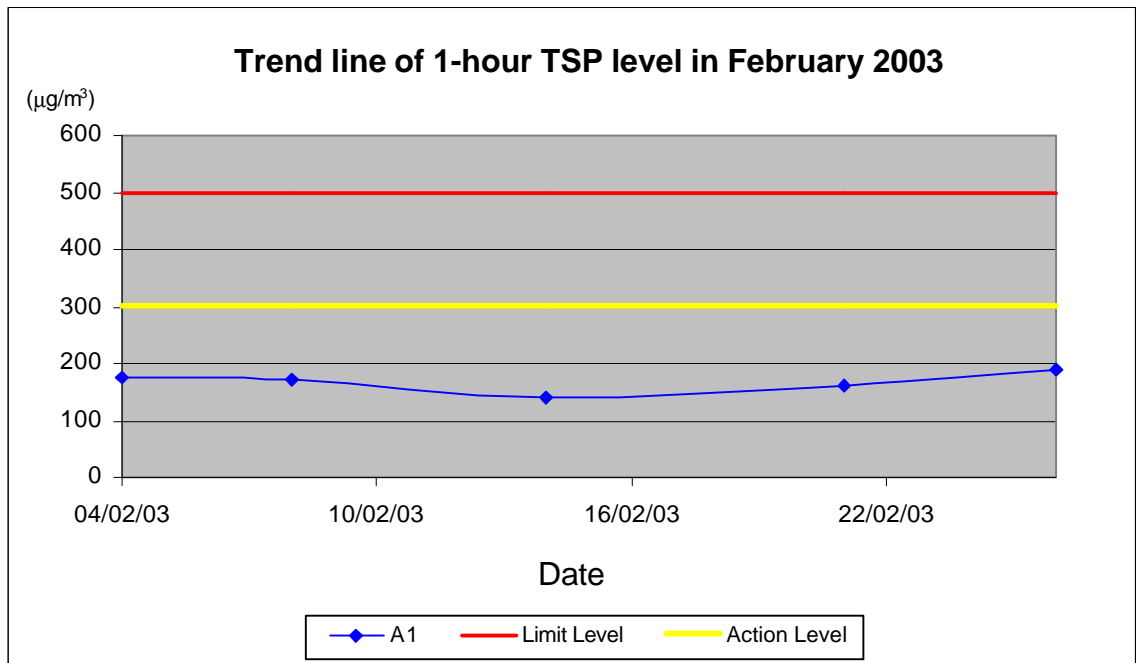
Figure 5-2 1-hour TSP monitoring results for February 2003
