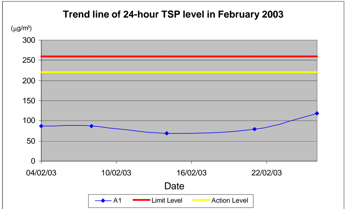
Figure 5-1 24-hour TSP monitoring results for February 2003
