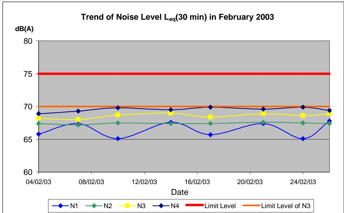
Figure 4-1 Daytime noise monitoring results for February 2003
