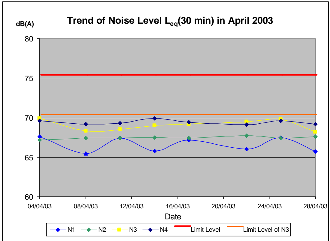
Figure 4-1 Daytime noise monitoring results for April 2003
