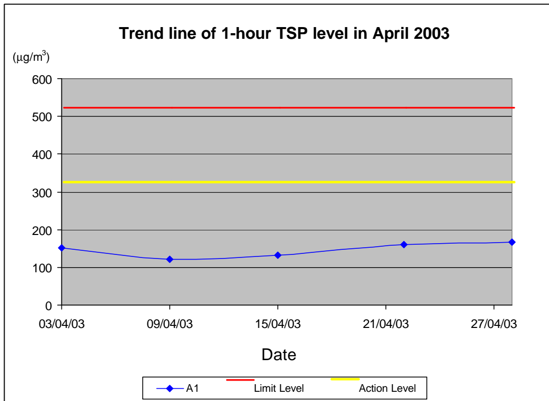
Figure 5-2 1-hour TSP monitoring results for April 2003
