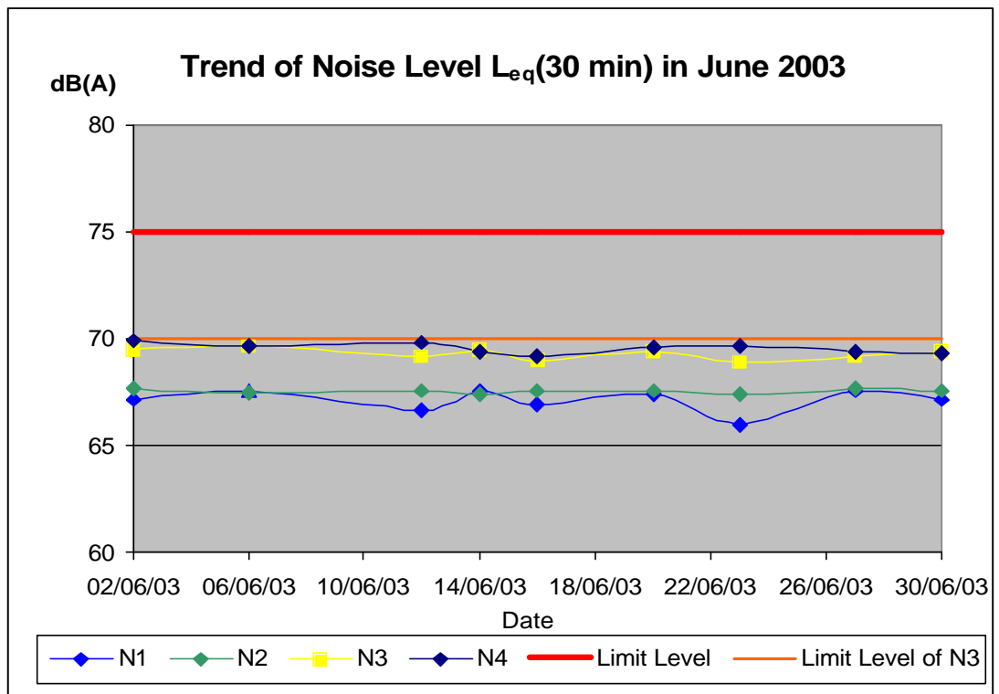
Figure 4-1 Daytime noise monitoring results for June 2003
