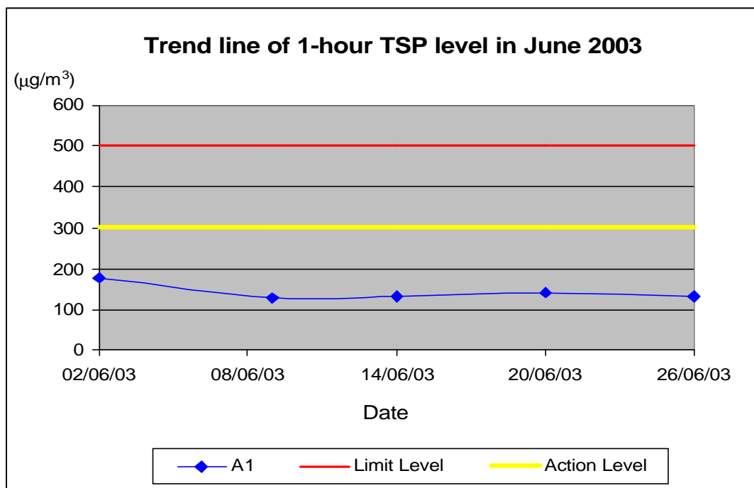
Figure 5-2 1-hour TSP monitoring results for June 2003
