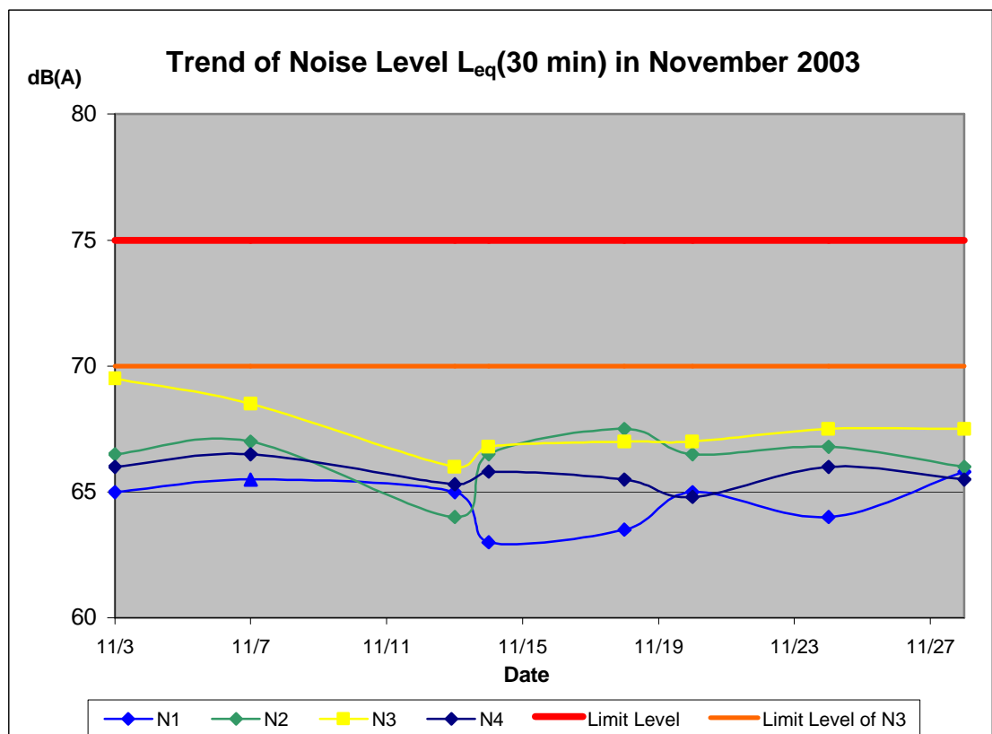
Figure 4-1 Daytime noise monitoring results for November 2003
