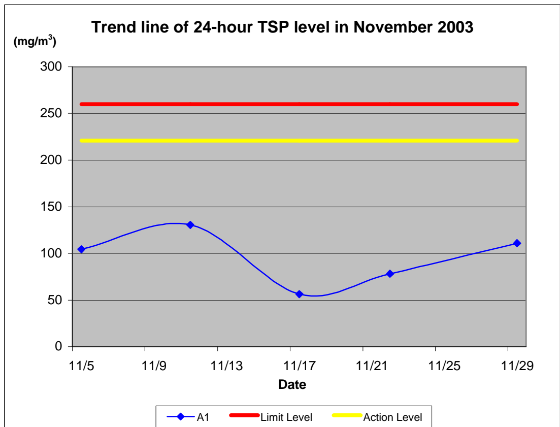
Figure 5-1 24-hour TSP monitoring results for November 2003
