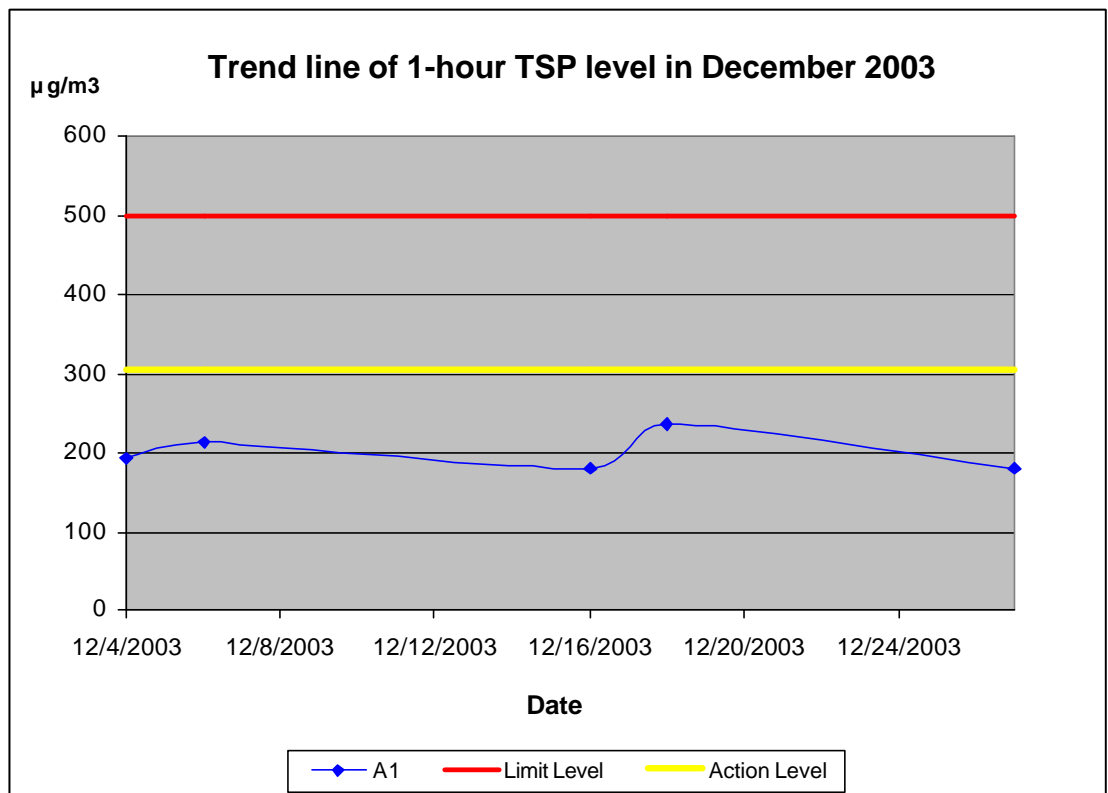
Figure 5-2 1-hour TSP monitoring results for December 2003
