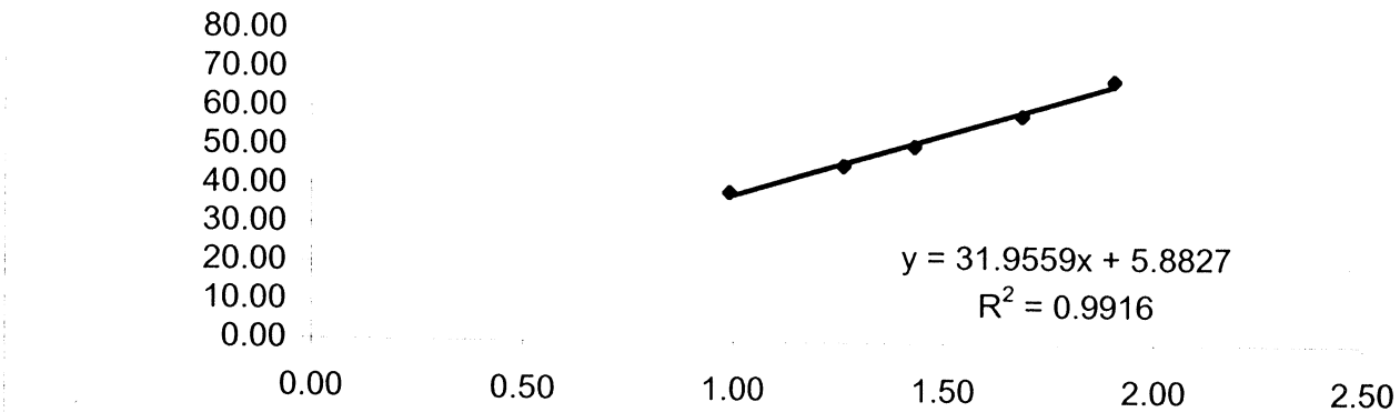
Calibration Curve
