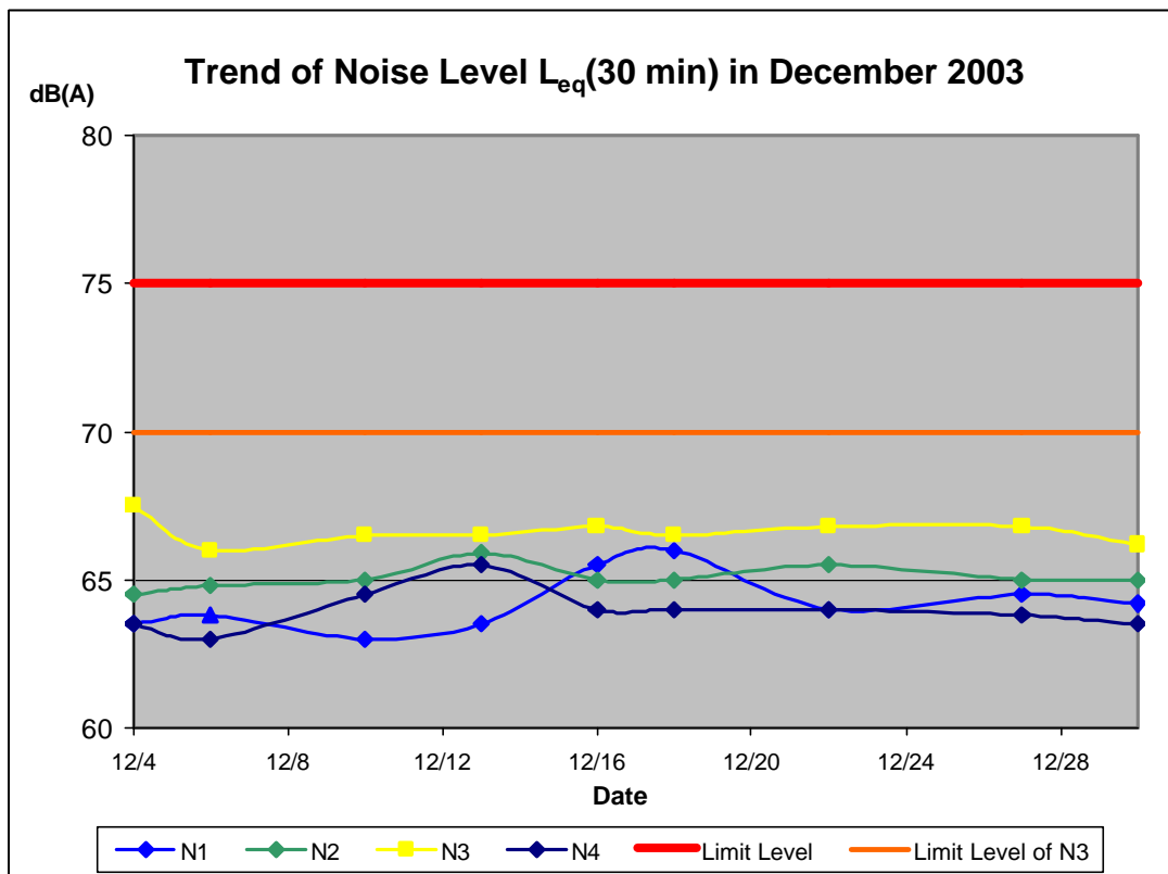
Figure 4-1 Daytime noise monitoring results for December 2003
