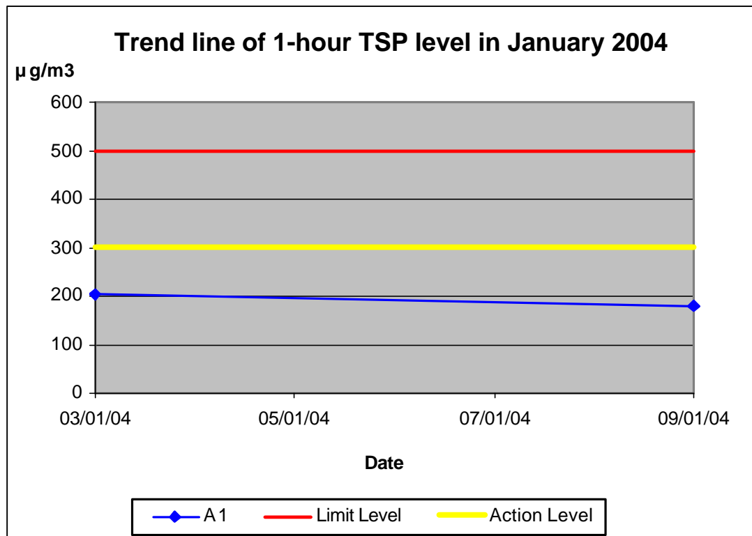
Figure 5-2 1-hour TSP monitoring results for January 2004
