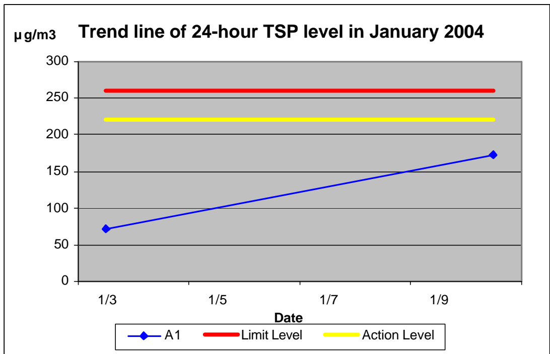
Figure 5-1 24-hour TSP monitoring results for January 2004
