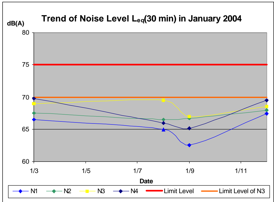
Figure 4-1 Daytime noise monitoring results for January 2004
