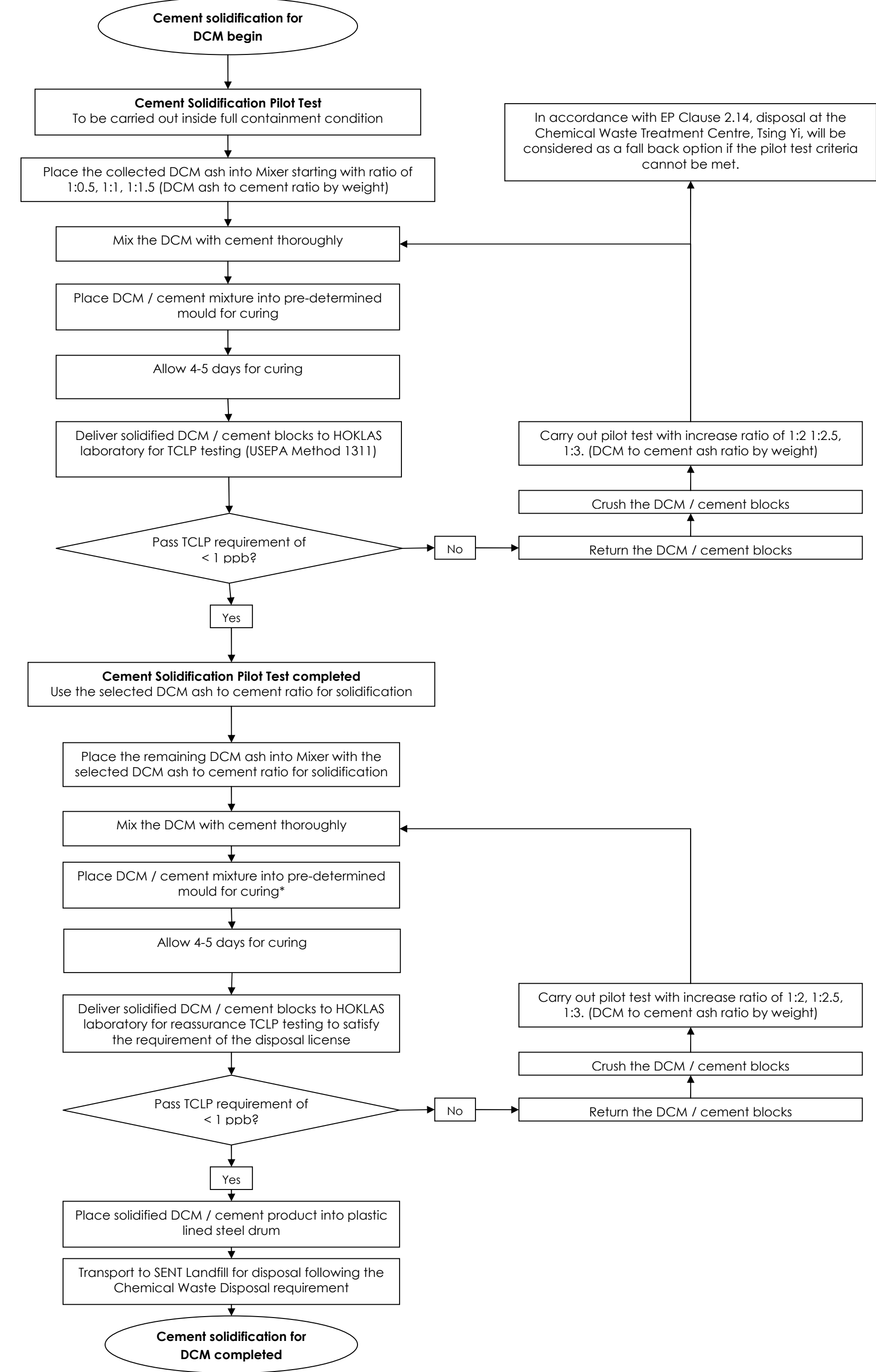
Work Flow Diagram for Cement Solidification (Ash contents within ash bunker) (where tested dioxin levels are more than 1 ppb)
