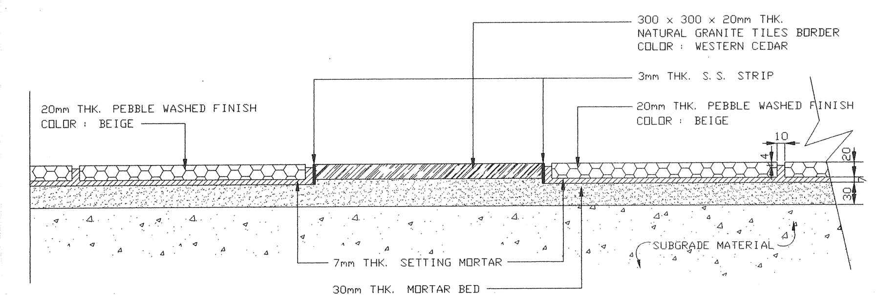
A PAVING DETAIL SCALE 1 : 5
