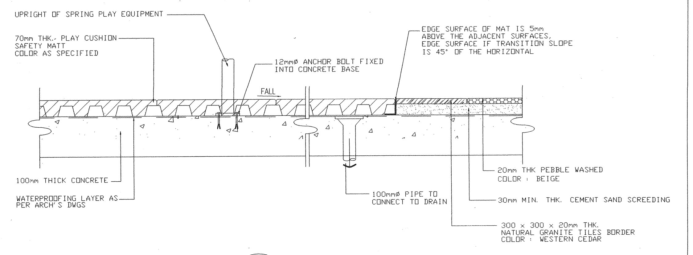
B SAFETY MATT DETAIL SCALE 1 : 10
