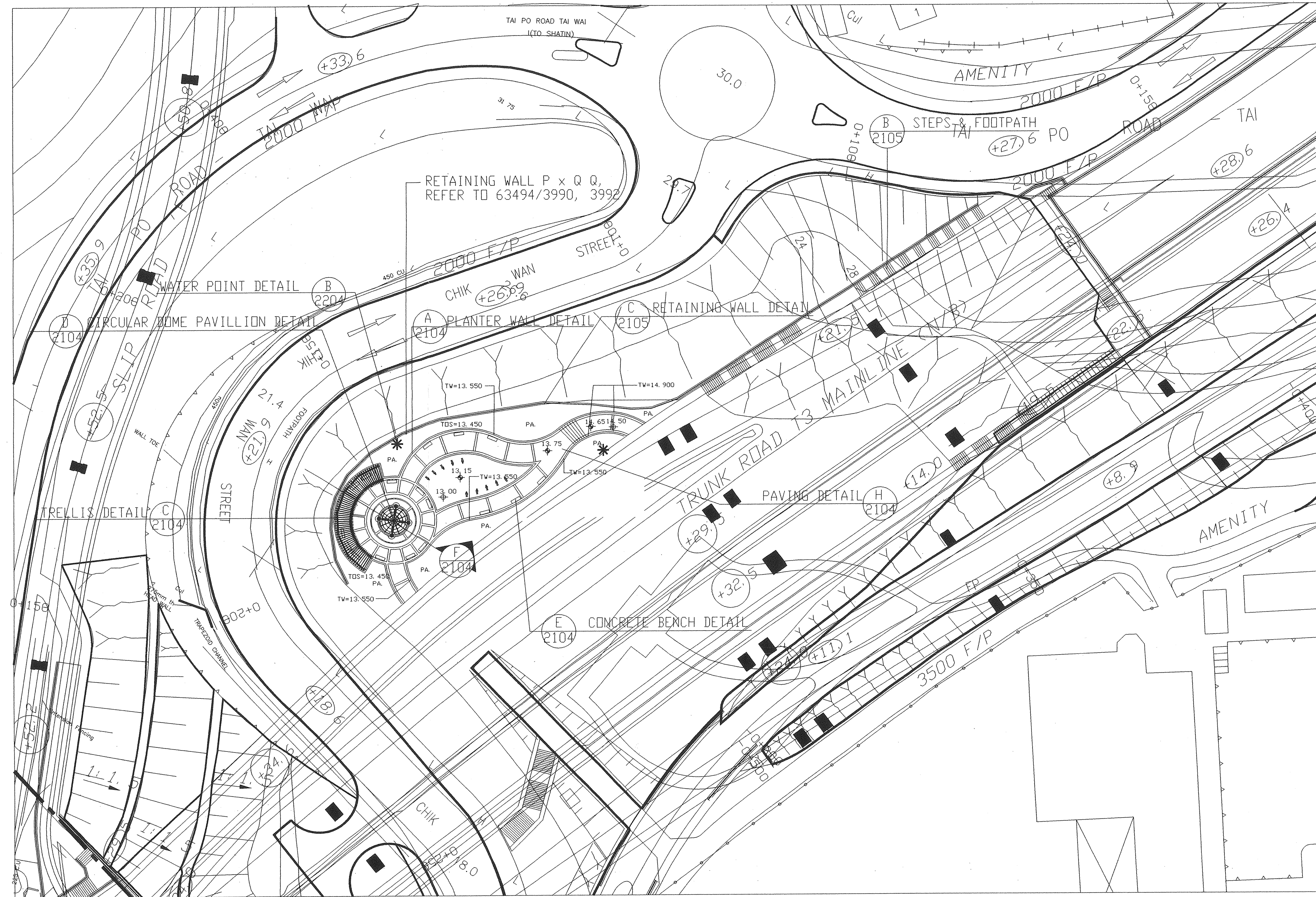
LANDSCAPE LAYOUT AND REFERENCE CALLOUT PLAN SCALE 1 : 400
