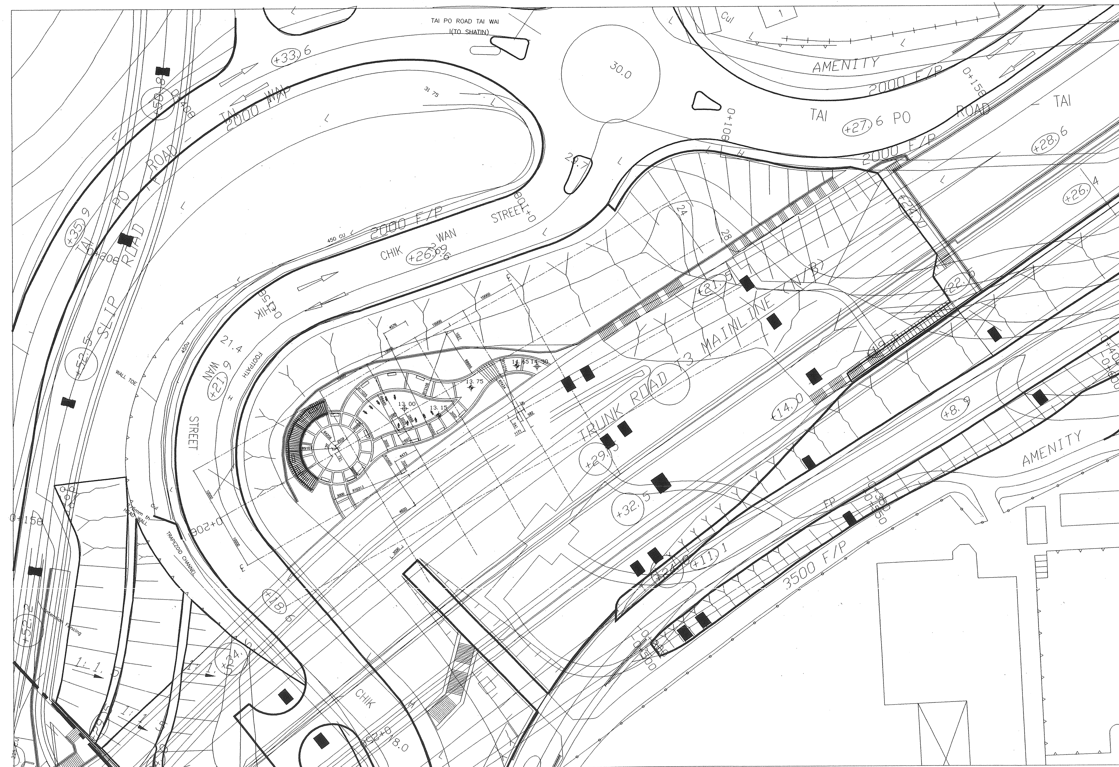
SETTING OUT PLAN SCALE 1 : 400
