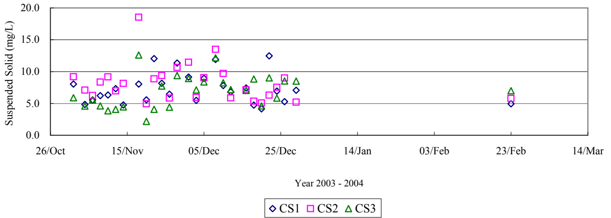
Suspended Solid (Depth Averaged) from CS1 to CS3 for Mid-Ebb Tide
