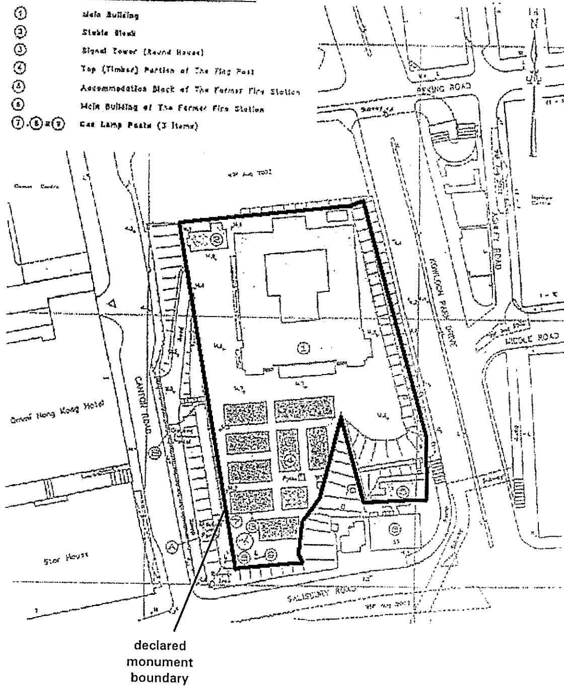
Figure 2.1 Location, site layout, historic buildings and structures to be preserved
