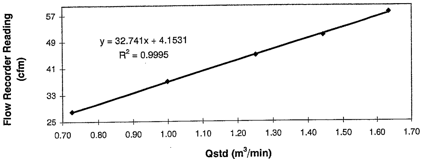
Sampler 8115 Calibration Curve Site: Tuen Mun 38 (AM-2) Date of Calibration: 06 September 2006
