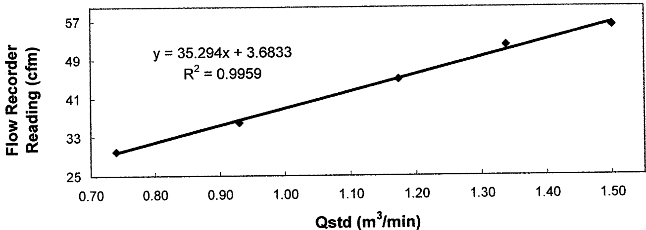
Sampler 9503 Calibration Curve Site: Tuen Mun 38 (AM-1) Date of Calibration: 08 May 2007
