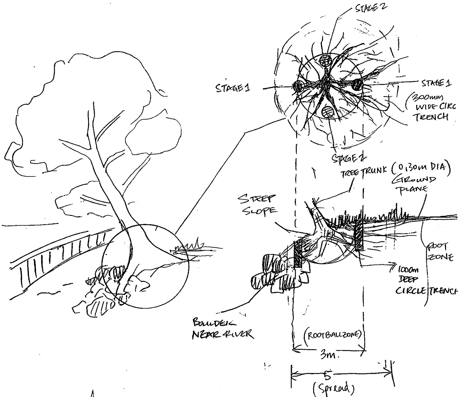
EXAMPLE OF ROOT PRUNING WORK FOR TREE NO. T234
