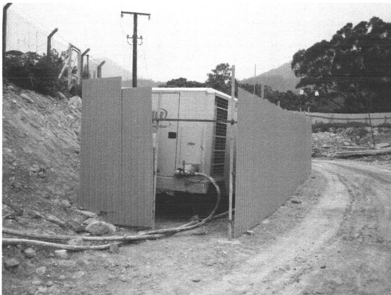
Photo 2: Erection of temporary noise barrier for the air compressor.
