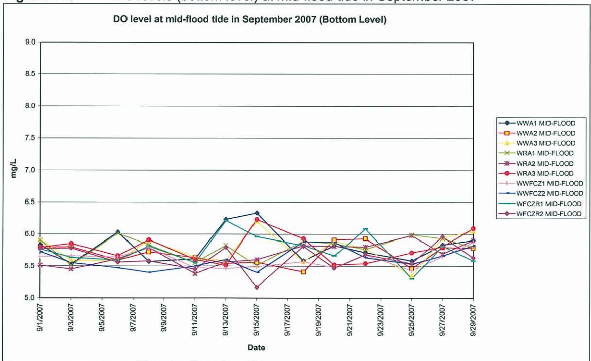
Figure 5-4: DO levels (bottom level) at mid-flood tide in September 2007
