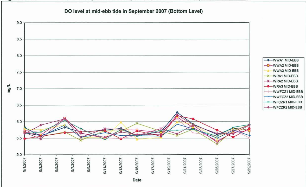
Figure 5-2: DO levels (bottom level) at mid-ebb tide in September 2007
