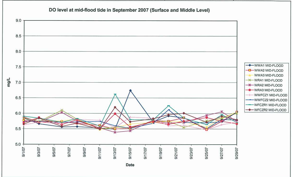
Figure 5-3: DO levels (surface and middle level) at mid-flood tide in September 2007
