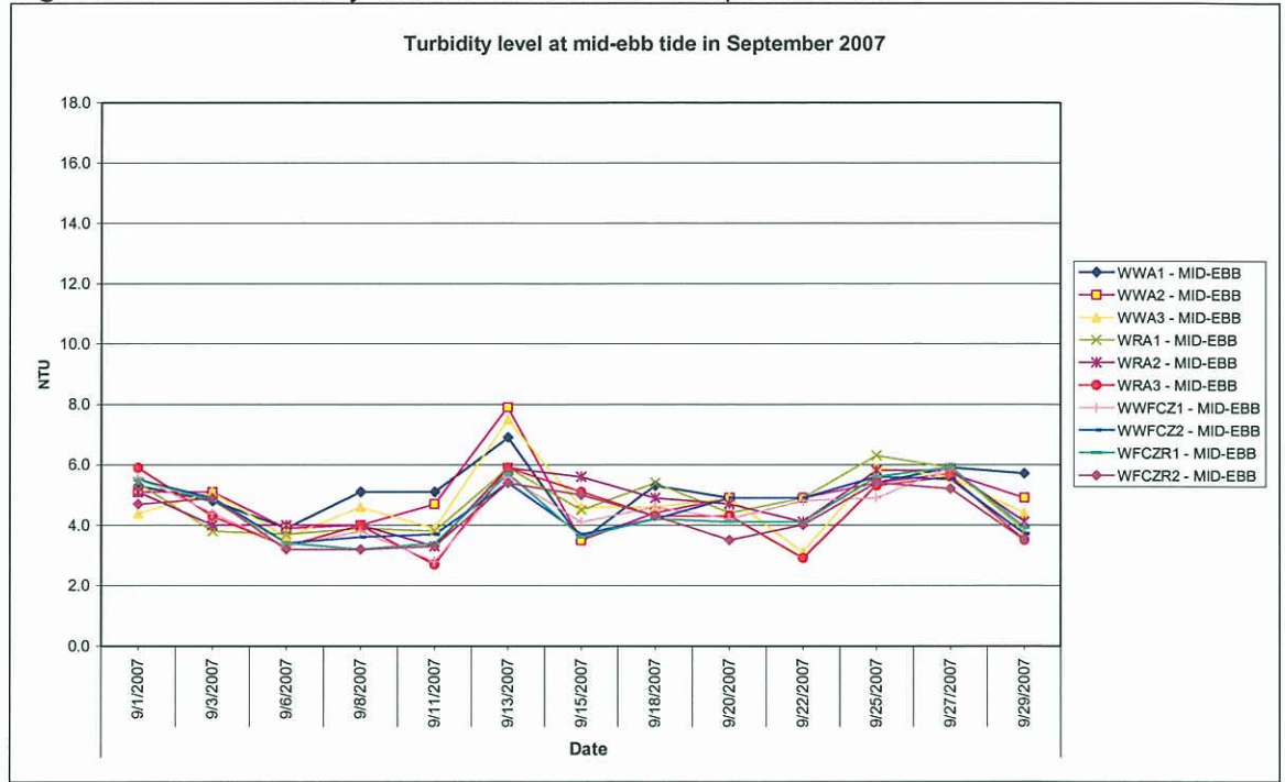
Figure 5-5: Turbidity levels at mid-ebb tide in September 2007
