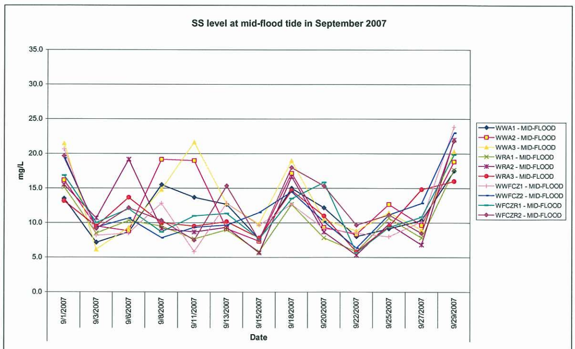
Figure 5-8: SS levels at mid-flood tide in September 2007
