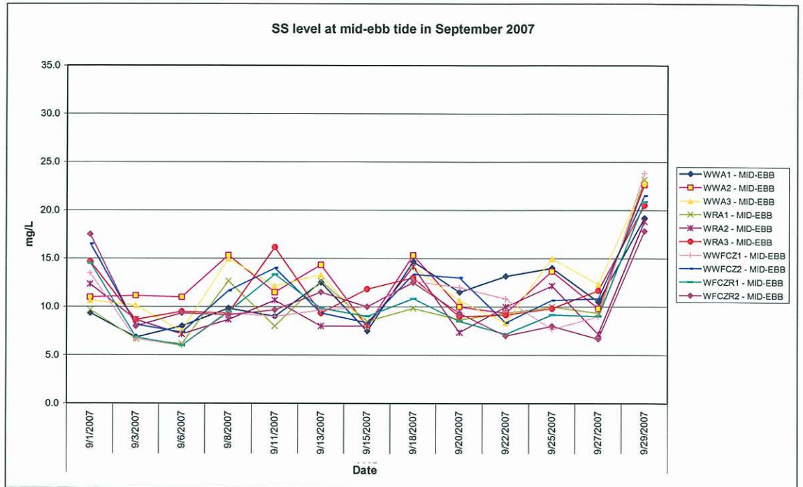
Figure 5-7: SS levels at mid-ebb tide in September 2007
