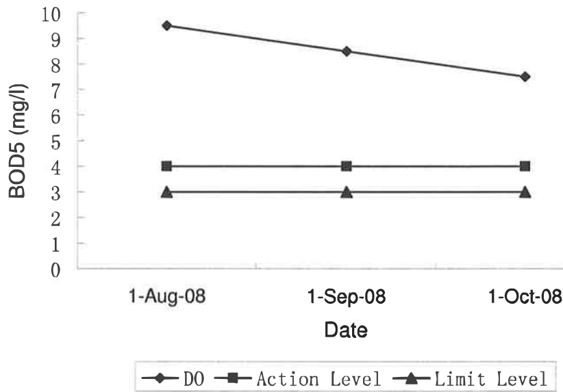
SkyCity Golf Lake Water Quality Monitoring DO at W4
