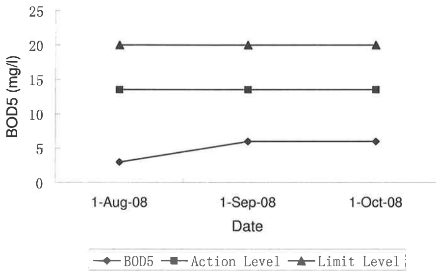
SkyCity Golf Lake Water Quality Monitoring BOD5 at W3
