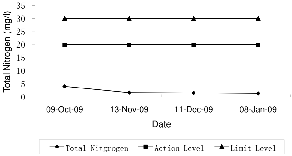
SkyCity Golf Lake Water Quality Monitoring Total Nitrogen at W3
