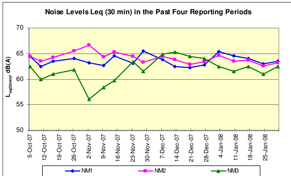
Figure 4-1: Graphical presentation of day-time noise levels
