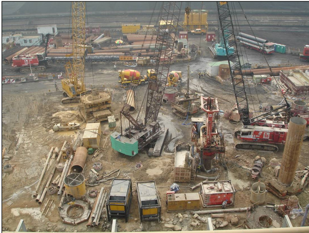
E. 1 Bored piling at the North Coal Stockyard
