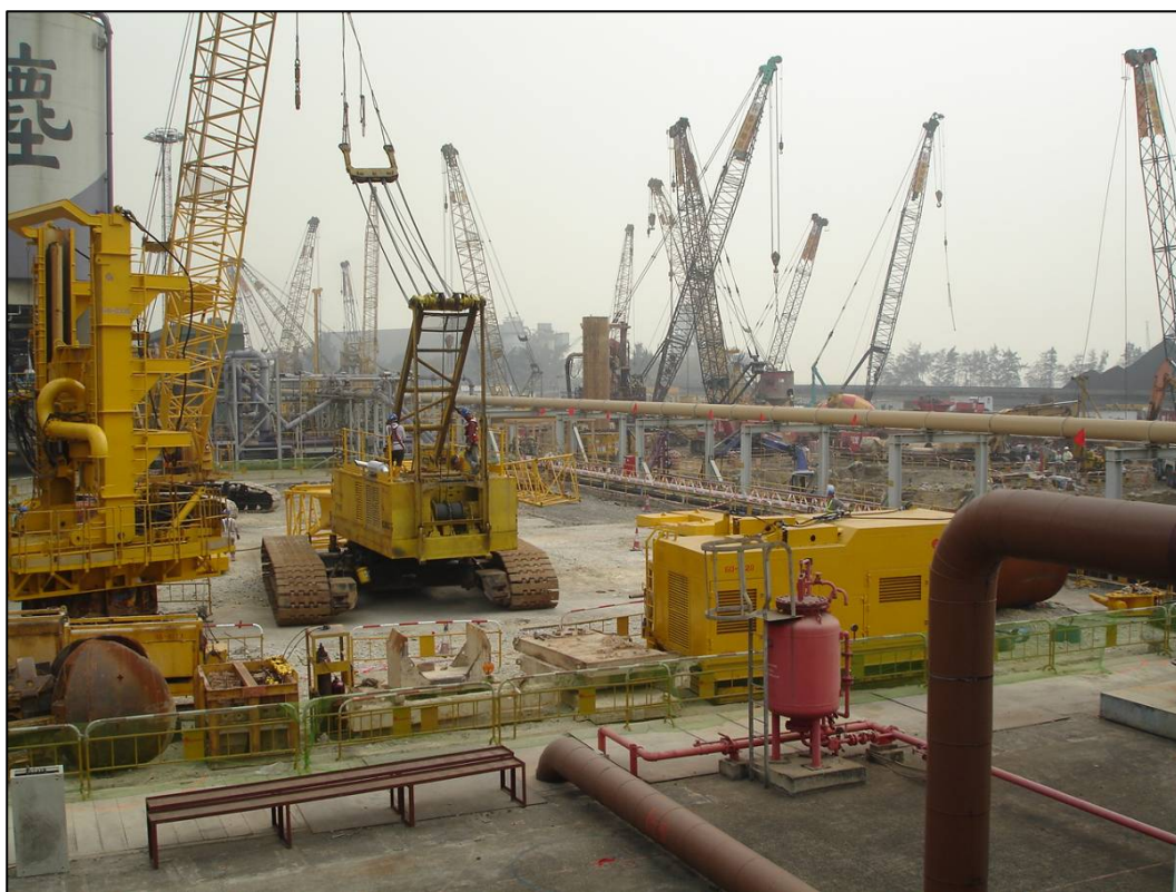
E. 2 Pre-drilling and extended trial pit excavation at the former D.G. Store area
