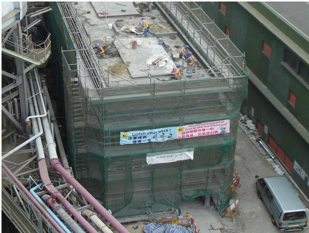
E.2 EC Power Distribution Centre (PDC) construction
