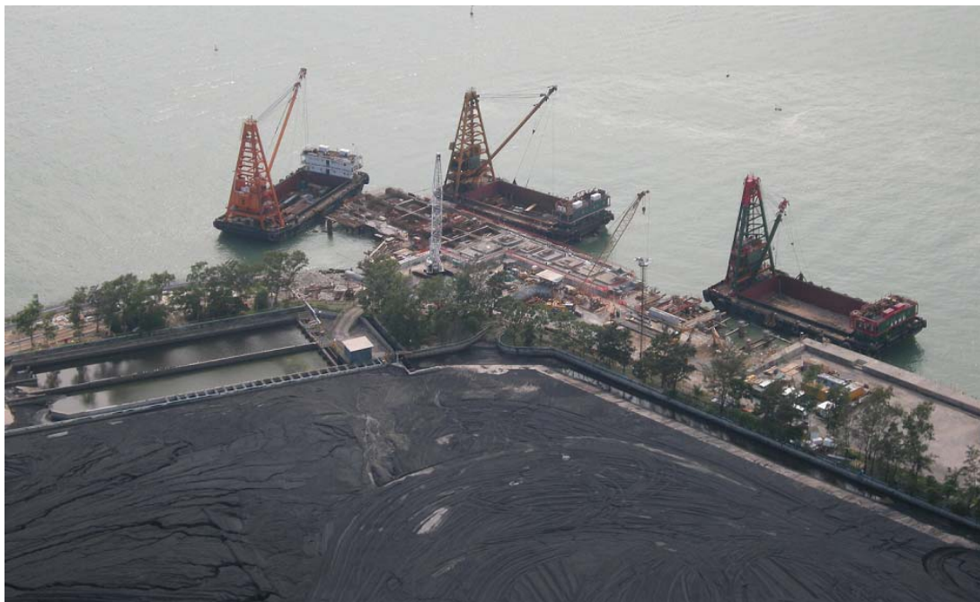
E.4 Material Handling Berth
