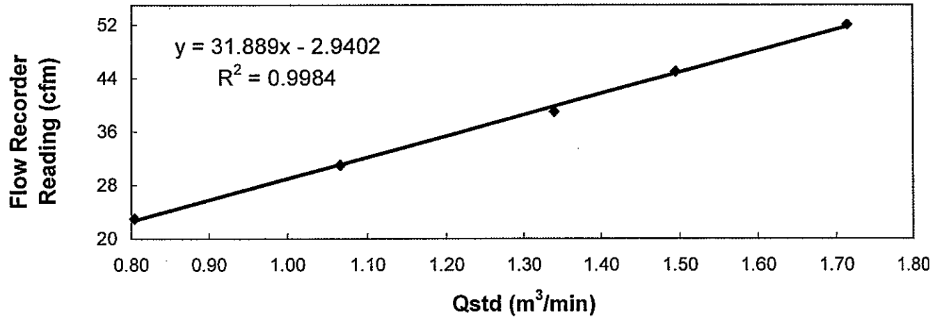
Sampler 9912 Calibration Curve Site: Sok Kwu Wan (AM-3) Date of Calibration: 11 June 2008
