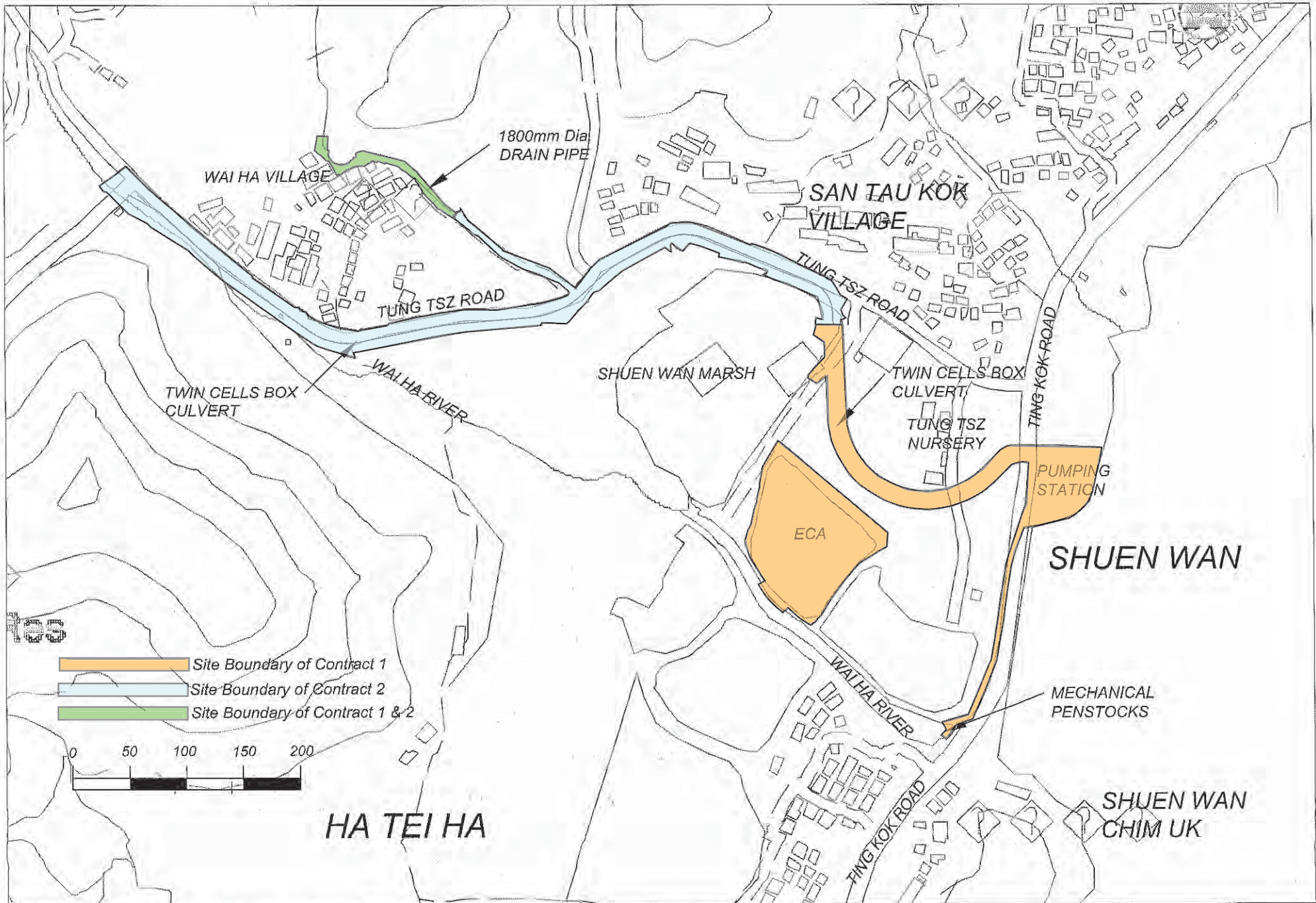
Site Location Plan of DSD Contract 1 and Contract at Shuen Wan
