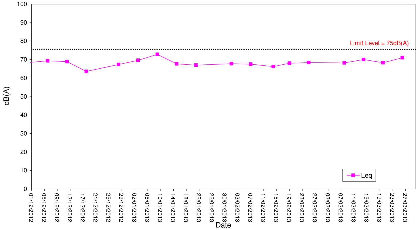
Noise Level for 30 min, dB(A), at NM8
