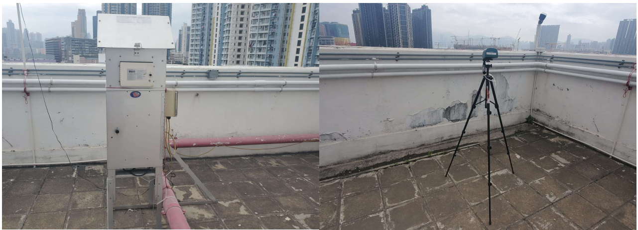
Measurement setup at AM2(A)
