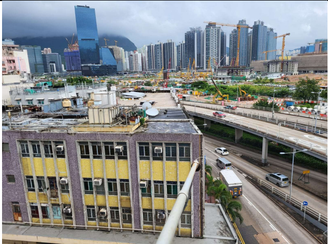
Measurement setup at M5(A)
