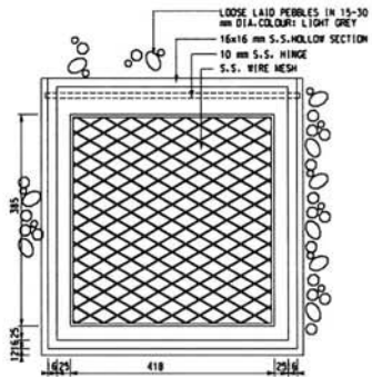
DETAIL OF TYPICAL DRAINAGE INSPECTION CHAMBER ① SCALE 1 : 5
