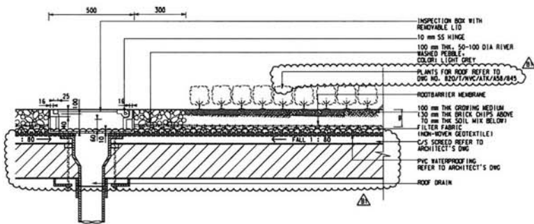
DETAIL OF TYPICAL DRAINAGE INSPECTION CHAMBER ② SCALE 1 : 10
