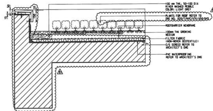
DETAIL OF PARAPET EDGE TREATMENT ③ SCALE 1 : 10
