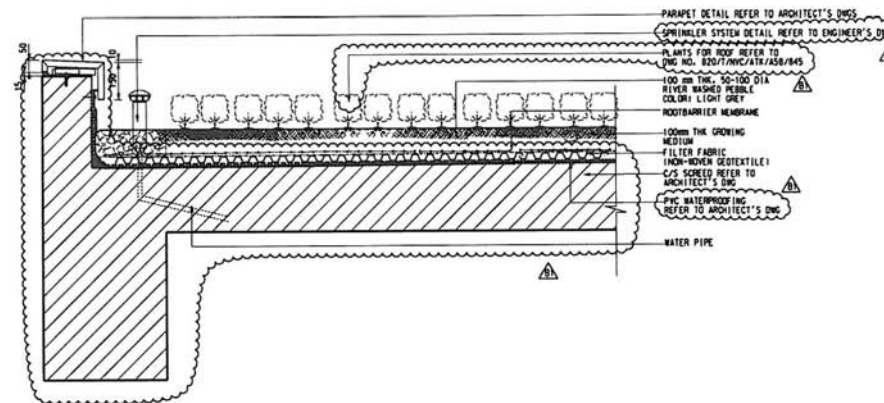
DETAIL OF TYPICAL PENETRATION OF ROOF-TOP UTILITIES ④ SCALE 1 : 10
