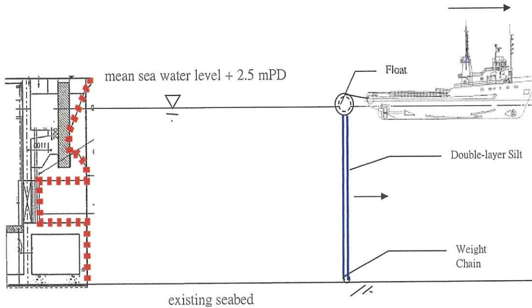
Sectional View A-A
