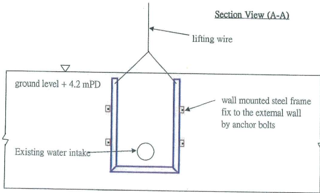
Elevation View
