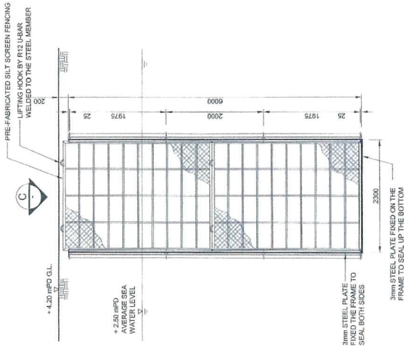
TYPICAL ARRANGEMENT OF SILT SCREEN FENCING INSTALLATION INTO THE WALL MOUNTED FRAME SCALE 1 : 50 (A3)
