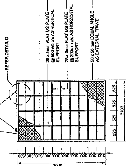
PRE-FABRICATED SILT SCREEN FENCING ( 2100mm WIDTH ) SCALE 1 : 50 (A3)
