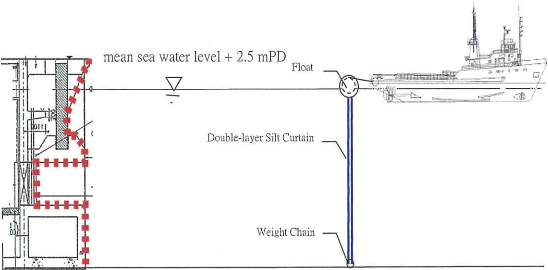
Sectional View A-A
