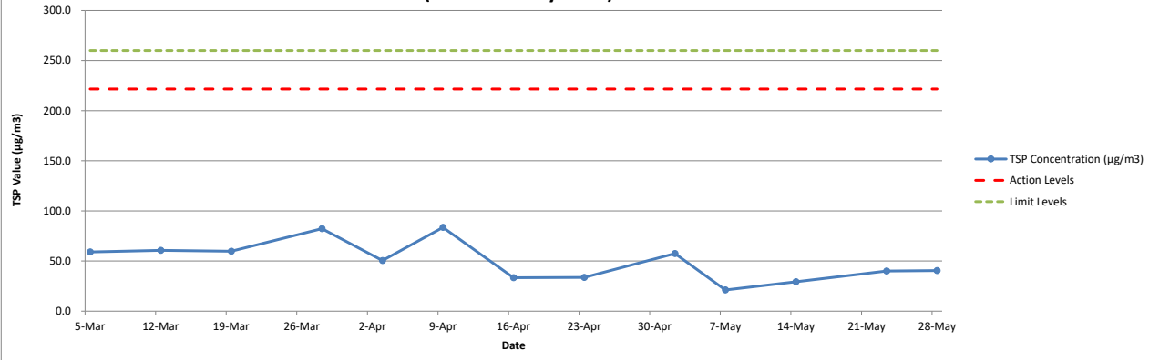
Impact Air Quality Monitoring (24-hr TSP) Result Plot at K11 (March to May 2018)
